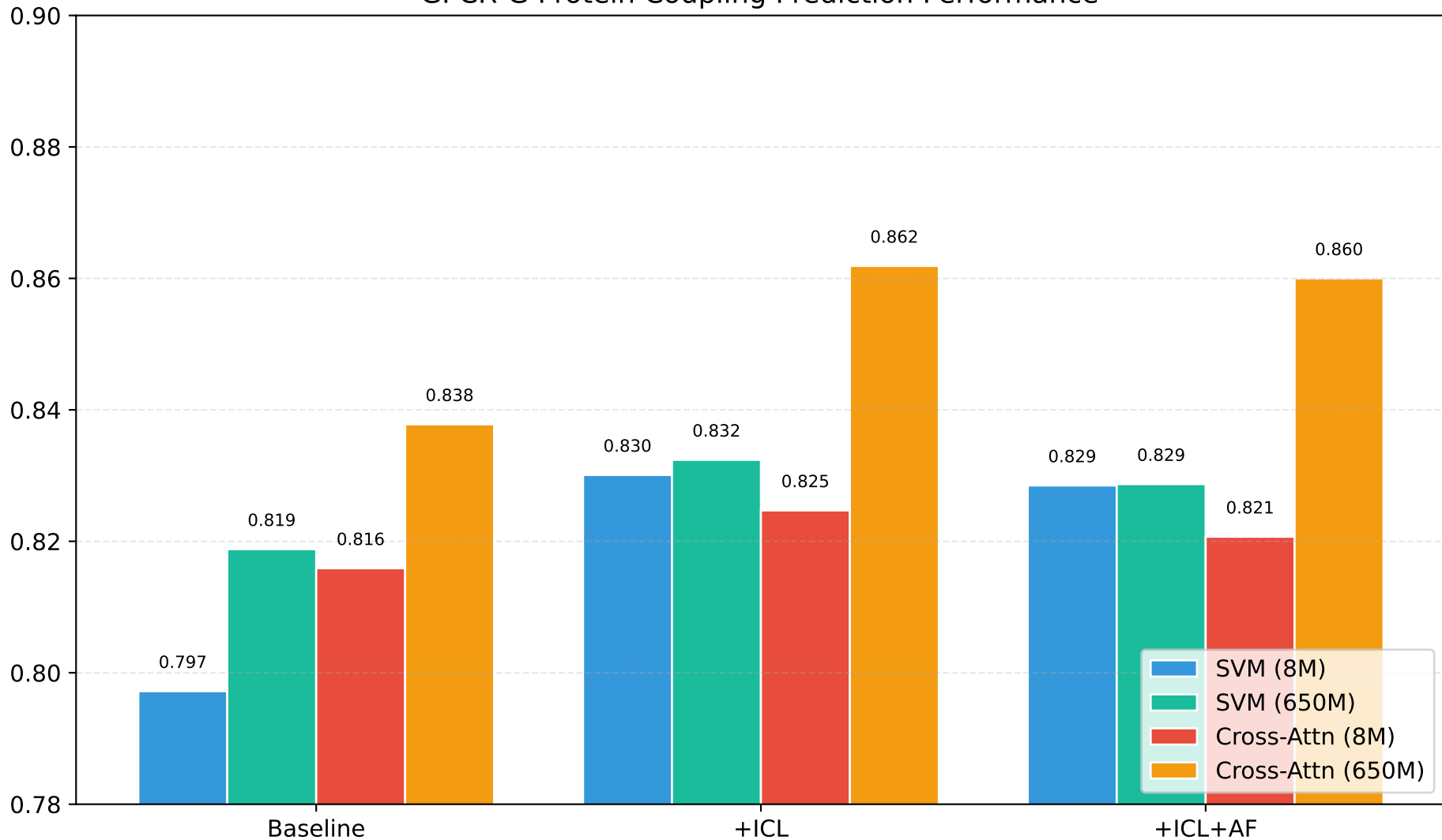
GPCR-G Protein Coupling Prediction Performance
