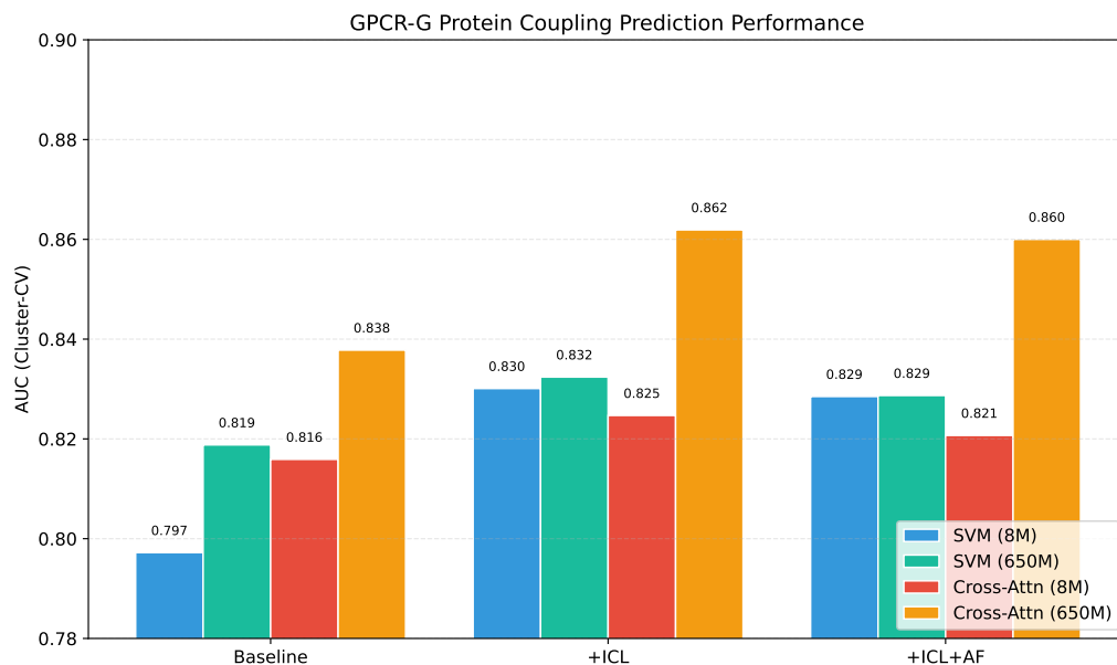
Figure 4: Performance comparison across model architectures and embedding scales under cluster-aware 5-fold cross-validation. Cross-attention with 650M + ICL achieves the best AUC (0.8619). The performance advantage of cross-attention over SVM widens from 8M ( \Delta\text{AUC} = +0.006 ) to 650M ( \Delta\text{AUC} = +0.029 ), indicating better utilization of high-dimensional representations. Error bars: \pm 1 std across 5 folds.
