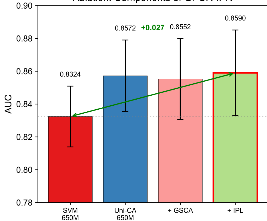
Ablation: Components of GPCR-IPN
