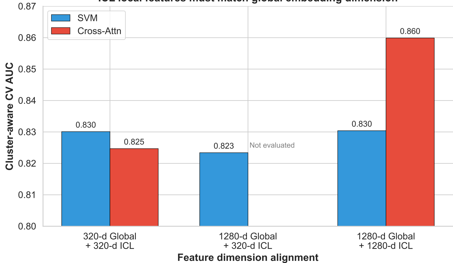
ICL local features must match global embedding dimension
