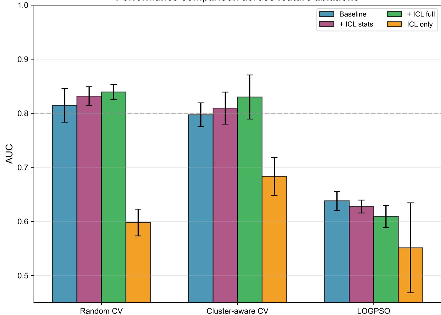
Performance comparison across feature ablations
