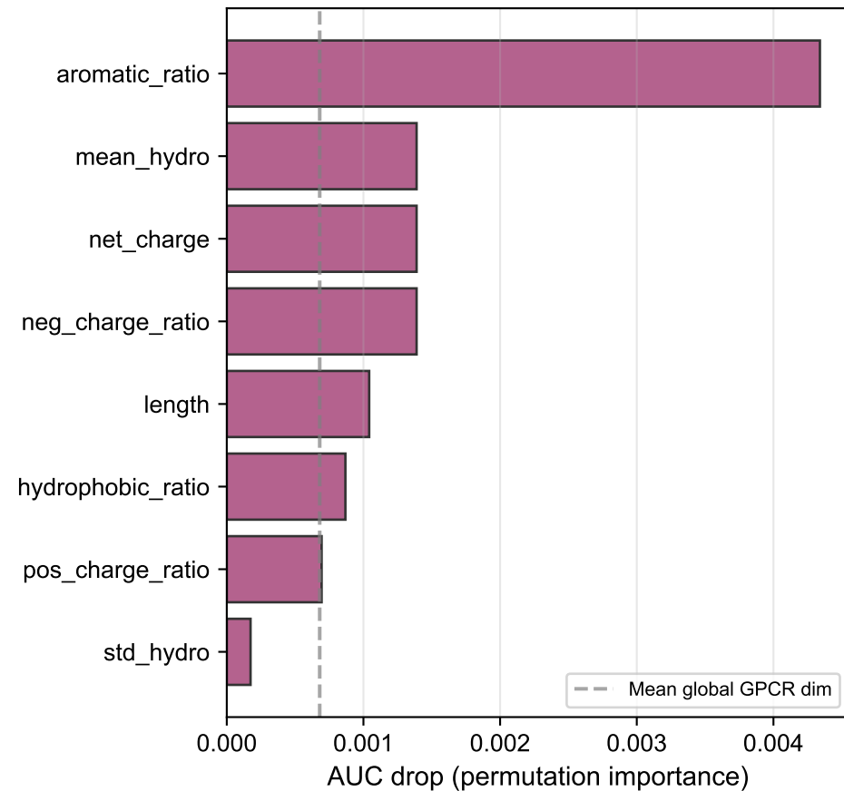
ICL2 statistics
