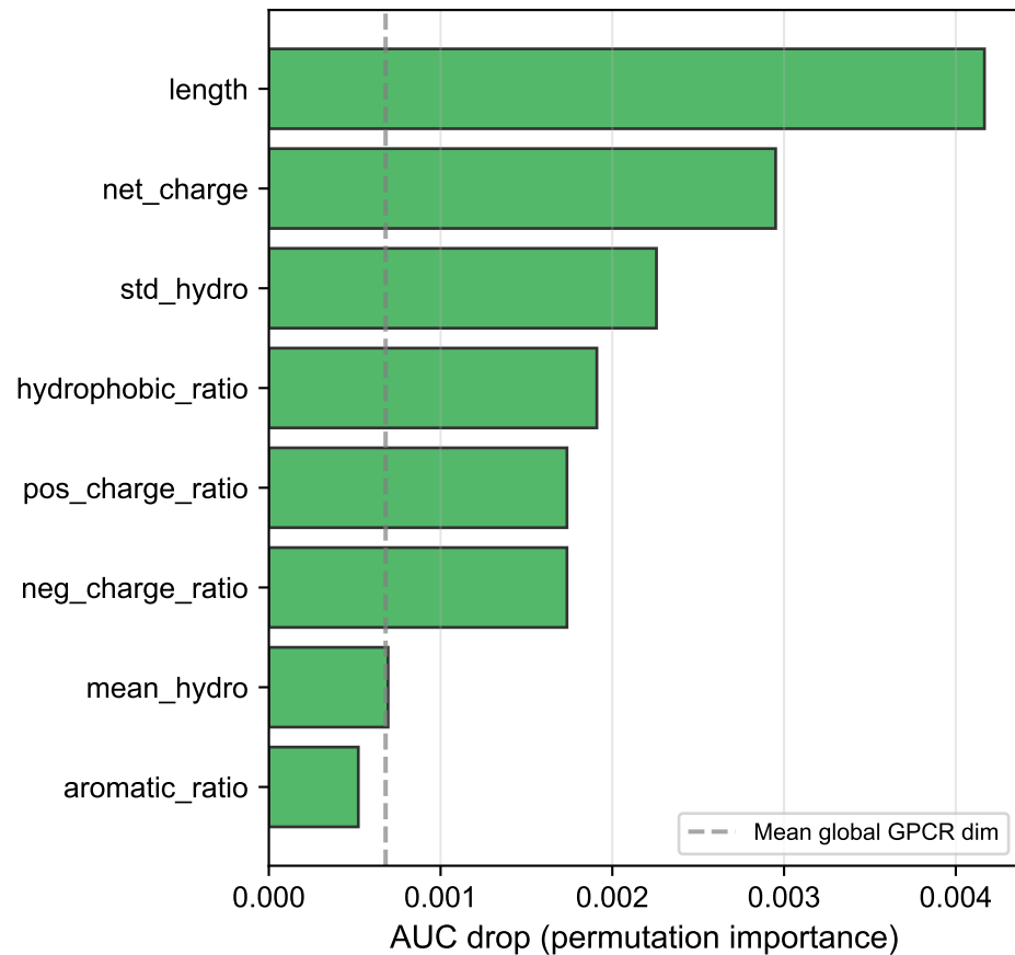
ICL3 statistics
