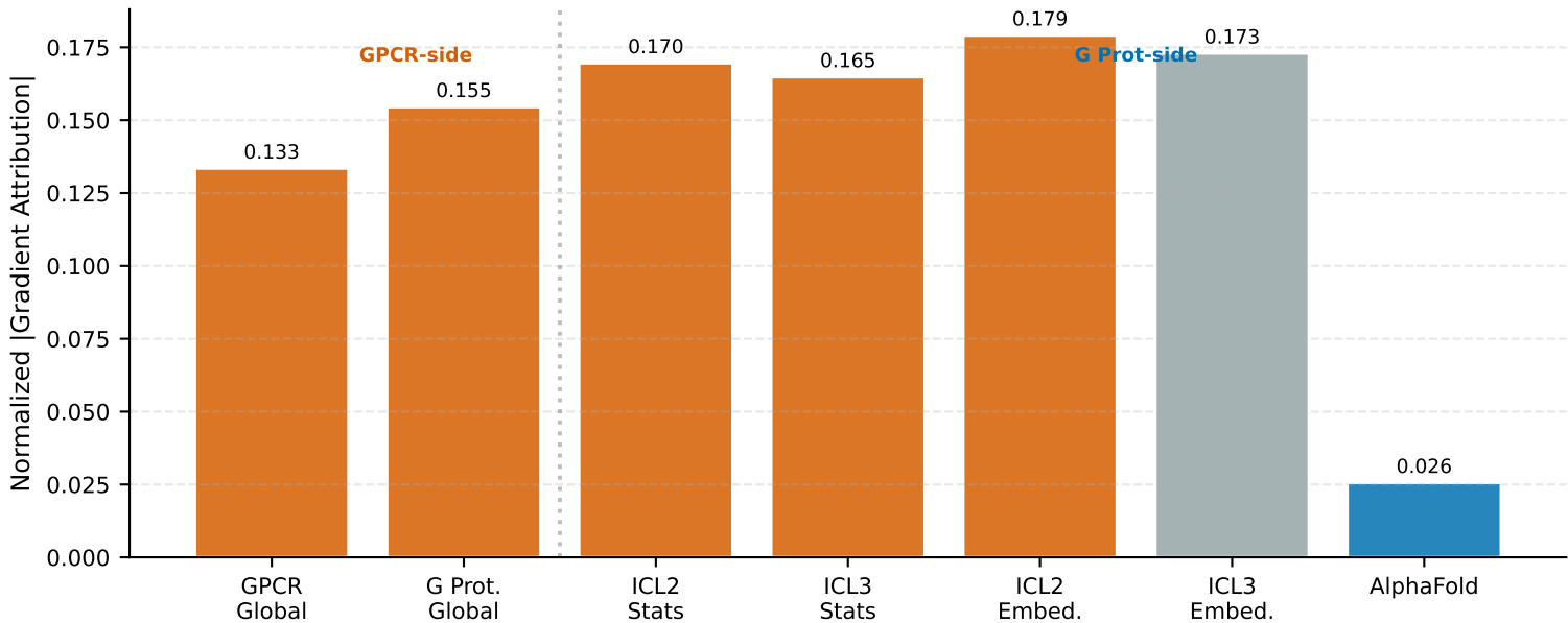
Feature Group Importance (Cross-Attention 650M)
