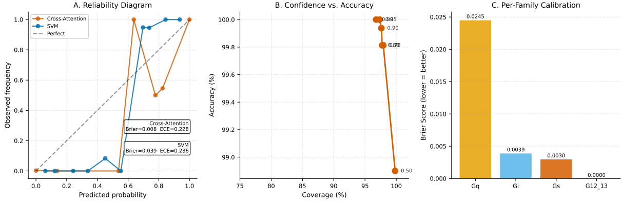
Figure 2: Model calibration and reliability. (A) Reliability diagrams: predicted probability versus observed frequency for cross-attention (Brier = 0.008) and SVM (Brier = 0.039). Perfect calibration indicated by dashed diagonal. (B) Accuracy versus coverage at increasing confidence thresholds. (C) Per-family Brier scores and expected calibration error (ECE).
