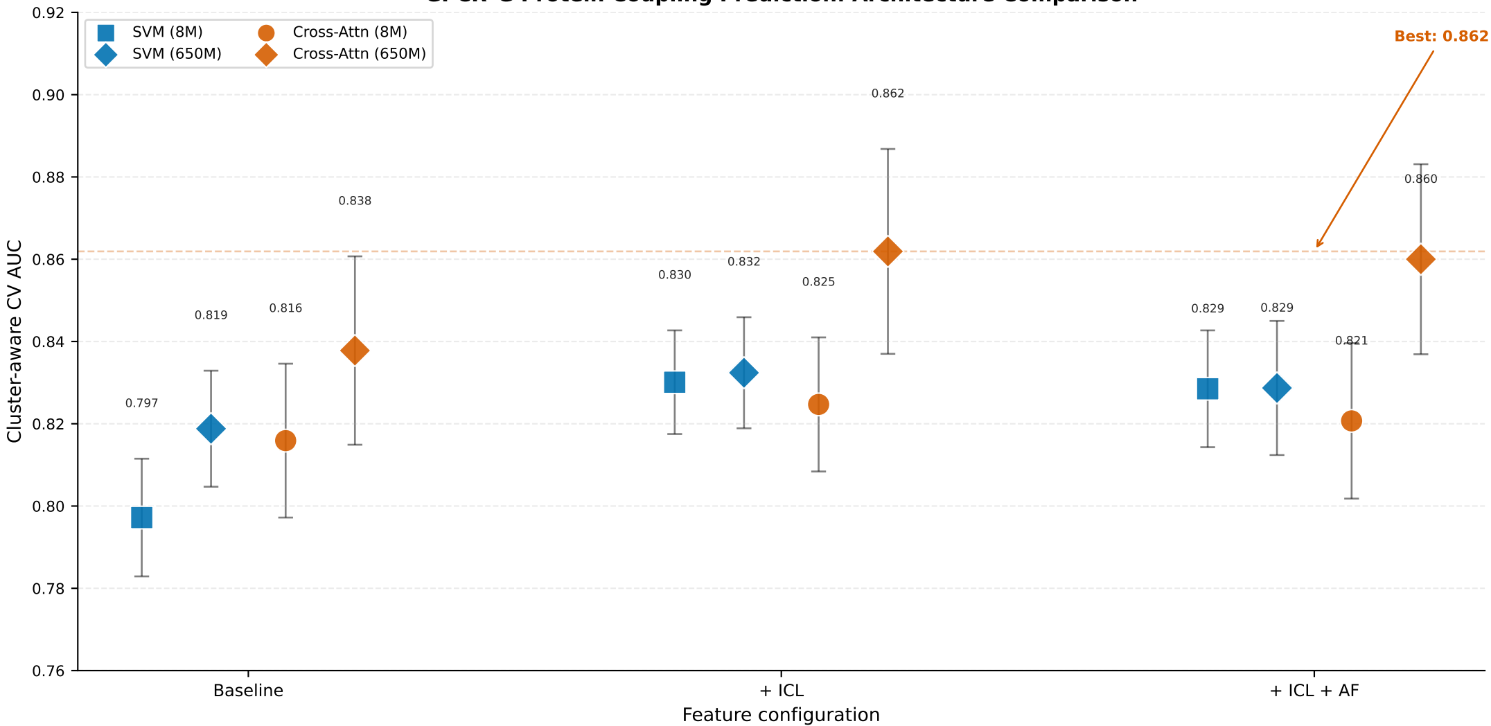
GPCR-G Protein Coupling Prediction: Architecture Comparison
