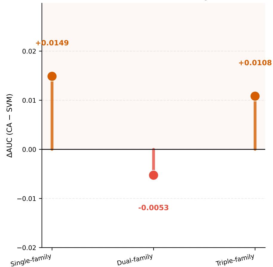
Cross-Attention Advantage
