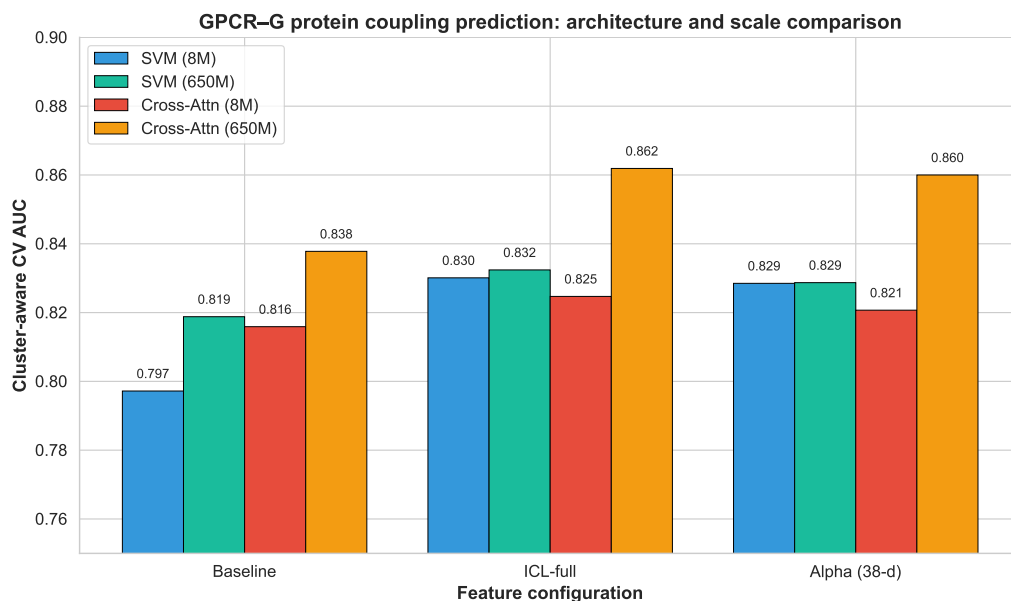
Figure 2: Cluster-aware CV AUC comparison across all model configurations. Cross-attention with 650M embeddings achieves the best performance (0.8619). SVM performance plateaus at \sim 0.833 regardless of embedding scale.
