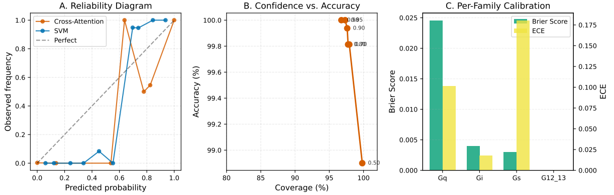
Figure 2: Model calibration and reliability. (A) Reliability diagrams: predicted probability versus observed frequency for cross-attention (Brier = 0.008) and SVM (Brier = 0.039). Perfect calibration indicated by dashed diagonal. (B) Accuracy versus coverage at increasing confidence thresholds. (C) Per-family Brier scores and expected calibration error (ECE).
