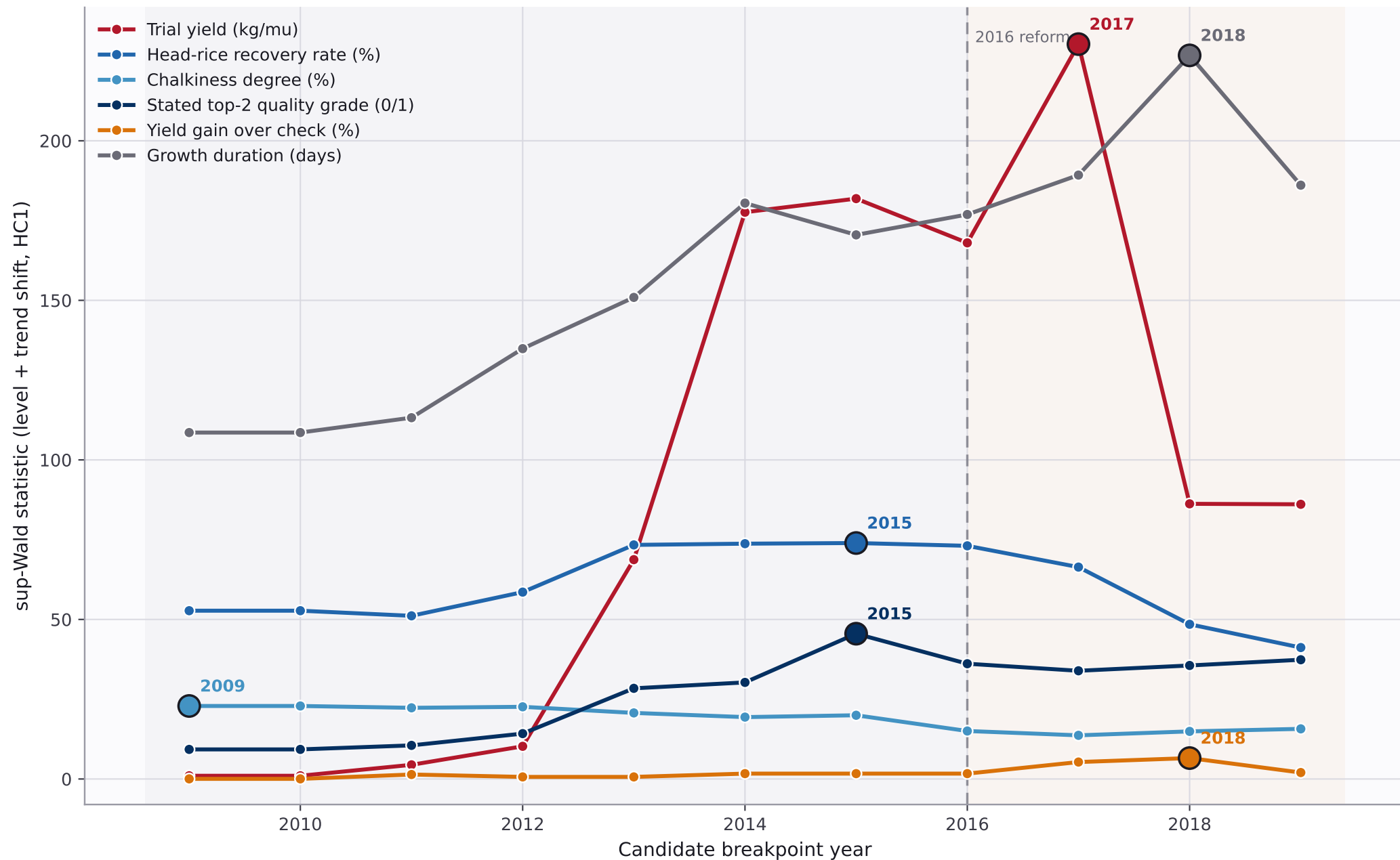
Fig. 4. Unknown-breakpoint (sup-Wald) scan by trait, national arm-1/arm-2 layer 2005-2022
