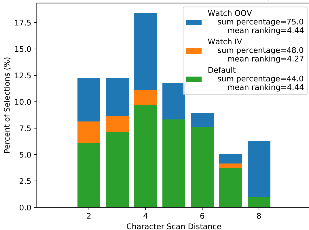
Character Scan Distance Distribution for Top 7
