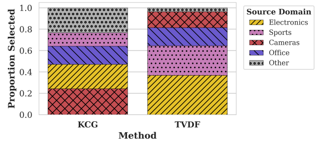
Figure R1: Analysis of out-of-domain sample selection for the Computers target domain from WDC using the KCG and TVDF methods.
