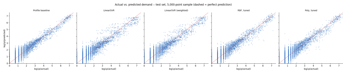
Figure 9: Actual vs. predicted demand, test set, all five community-area models (baseline, pooled LinearSVR, demand-weighted LinearSVR, tuned RBF, tuned polynomial), log1p scale.
