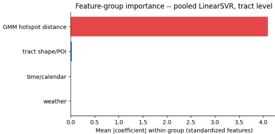
Figure 4: Mean |coefficient| by feature group. Hotspot distance versus time/calendar and weather is the clearest single illustration of the pooling-collapses-to-a-per-unit-constant finding described above.
