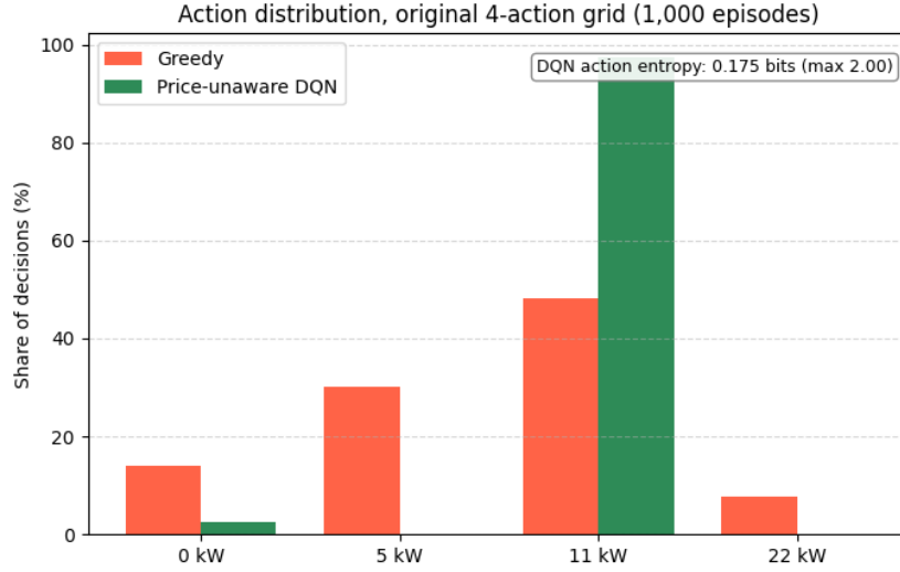
Figure 21: Action distribution on the original 4-action grid, 1,000 episodes (price-unaware DQN retrained with the notebook’s original hyperparameters and seed for this comparison). Greedy spreads its decisions across all four power levels, while the DQN collapses onto 11 kW in 97% of them – the degenerate habit that the refined grid in Table 18 corrects.
