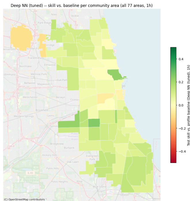
Figure 15: Tuned deep NN per-area skill vs. the profile baseline, all 77 community areas, 1-hour resolution.
