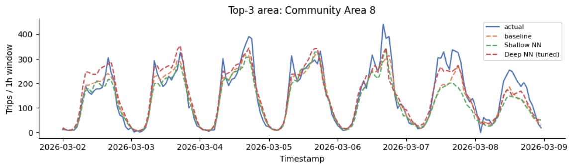
Figure 14: Neural-network March-week demand, Community Area 8, 1-hour resolution.
