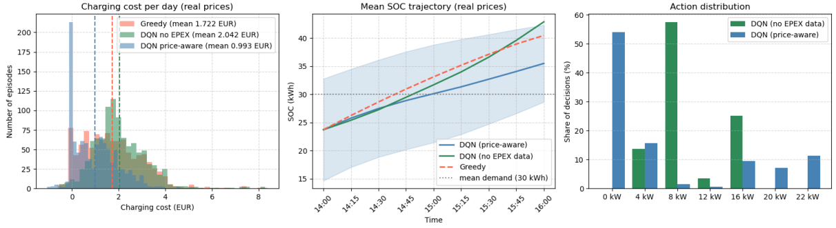
Figure 22: Charging-cost distribution, mean SOC trajectory, and action mix under EPEX prices, refined grid, 1,000 paired episodes. The EPEX DQN’s cost mass sits near zero and its SOC trajectory runs lowest of the three policies, consistent with its lower success rate in Table 19; the price-unaware DQN concentrates on 8 kW and 16 kW, while the EPEX DQN uses more of the grid, including 0 kW.
