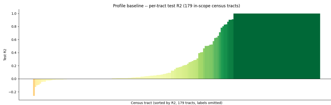
Figure 17: Profile baseline test R^2 per census tract, 4-hour resolution. Wider spread than the community-area version (Figure 5), consistent with more units competing for the same total demand.
