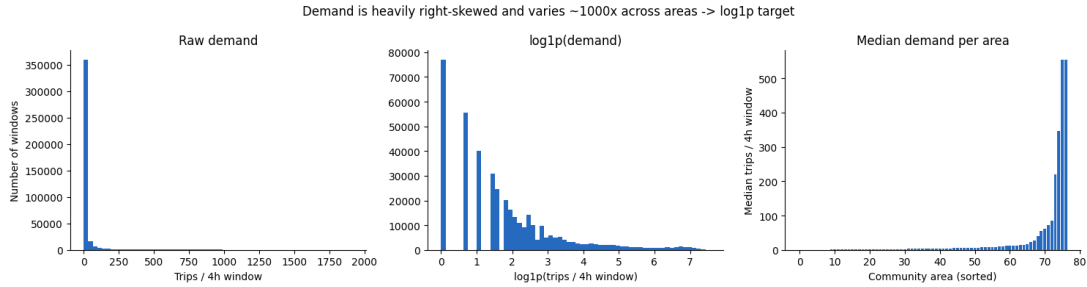
Figure 3: Raw per-window demand is heavily right-skewed, which is why both SVR and NN regress on \log1p(\text{count}) rather than raw counts.
