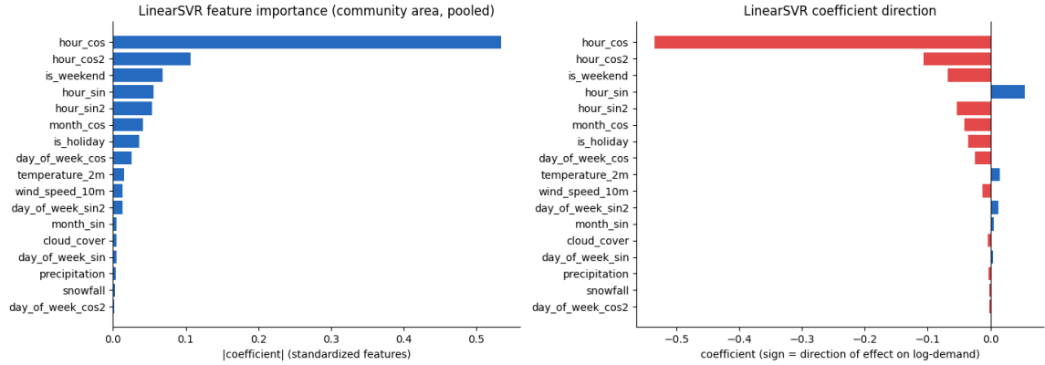
Figure 8: Pooled LinearSVR coefficients on the standardized features (community area, 4-hour). Left: magnitude (feature importance); right: sign. The calendar features – the hour-of-day harmonics above all, then weekend/holiday, weekday and month – dominate, while the weather variables rank lowest, with precipitation and snowfall near zero.
