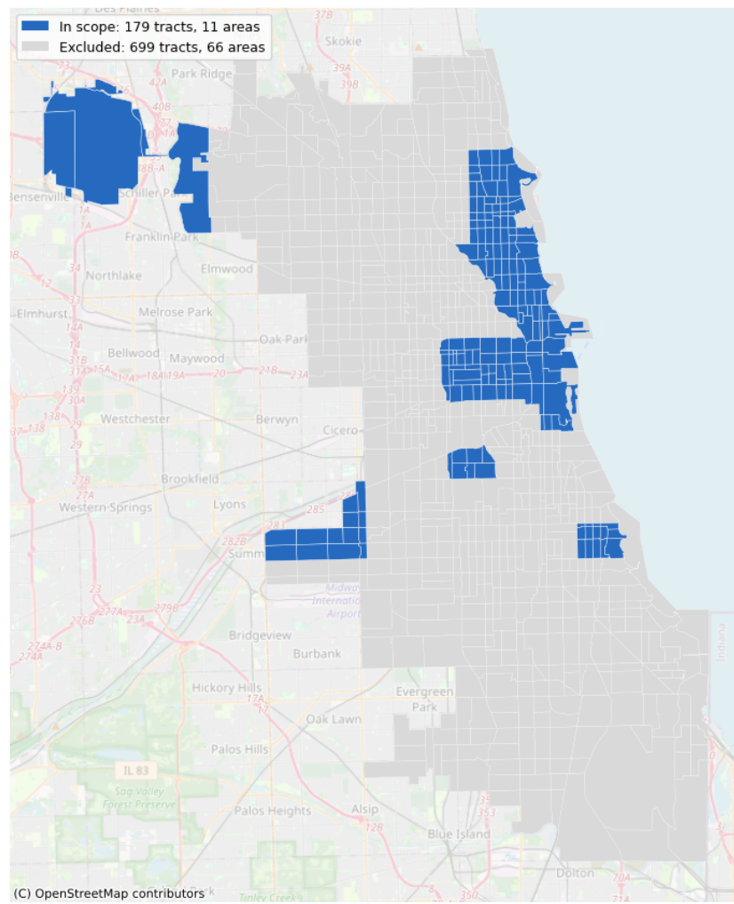
Figure 16: Scope map: the 179 of 878 census tracts with enough tract-precision data to support a tract-level model, across 11 community areas.
