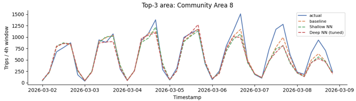
Figure 9: Actual, baseline and neural-network demand across the March evaluation week, Community Area 8 (highest demand), community area 4-hour resolution.
