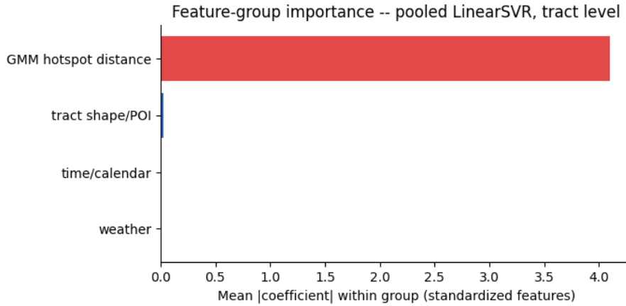
Figure 7: Mean |coefficient| by feature group. Hotspot distance versus time/calendar and weather is the clearest single illustration of the pooling-collapses-to-a-per-unit-constant finding described above.
