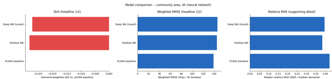
Figure 17: NN model comparison, community area, 4h: demand-weighted skill, weighted RMSE, and relative MAE for baseline, Shallow NN, and tuned Deep NN.
