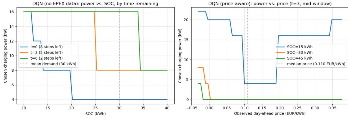
Figure 31: Learned charging policies as a function of state, refined grid. Left: the price-unaware DQN’s chosen power falls as SOC rises and as fewer steps remain, independent of price. Right: the EPEX DQN’s chosen power falls as price rises above the median (dotted line) and shifts up as SOC drops from 45 to 15 kWh, so urgency dominates price once charge is low.
