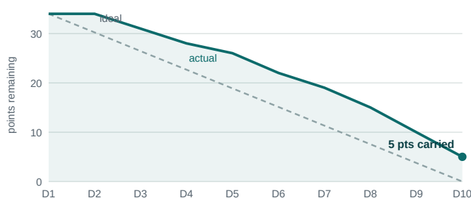
Sprint burndown (story points remaining)
