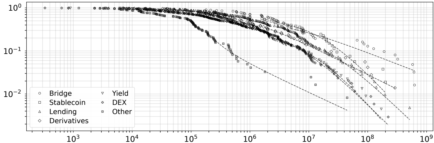
Empirical CCDF P(X \geq L)
