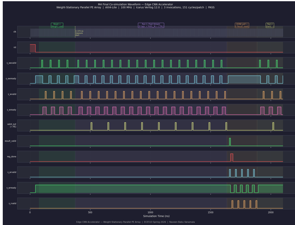
Figure 3: M4 co-simulation waveform — Reset+Weight Load → Run 1 pixel stream (9 taps, PIXEL_IN+CTRL) → DONE poll + 4 result reads → Run 2 start. t=375 ns marks measurement start; 151 cycles/patch measured.
