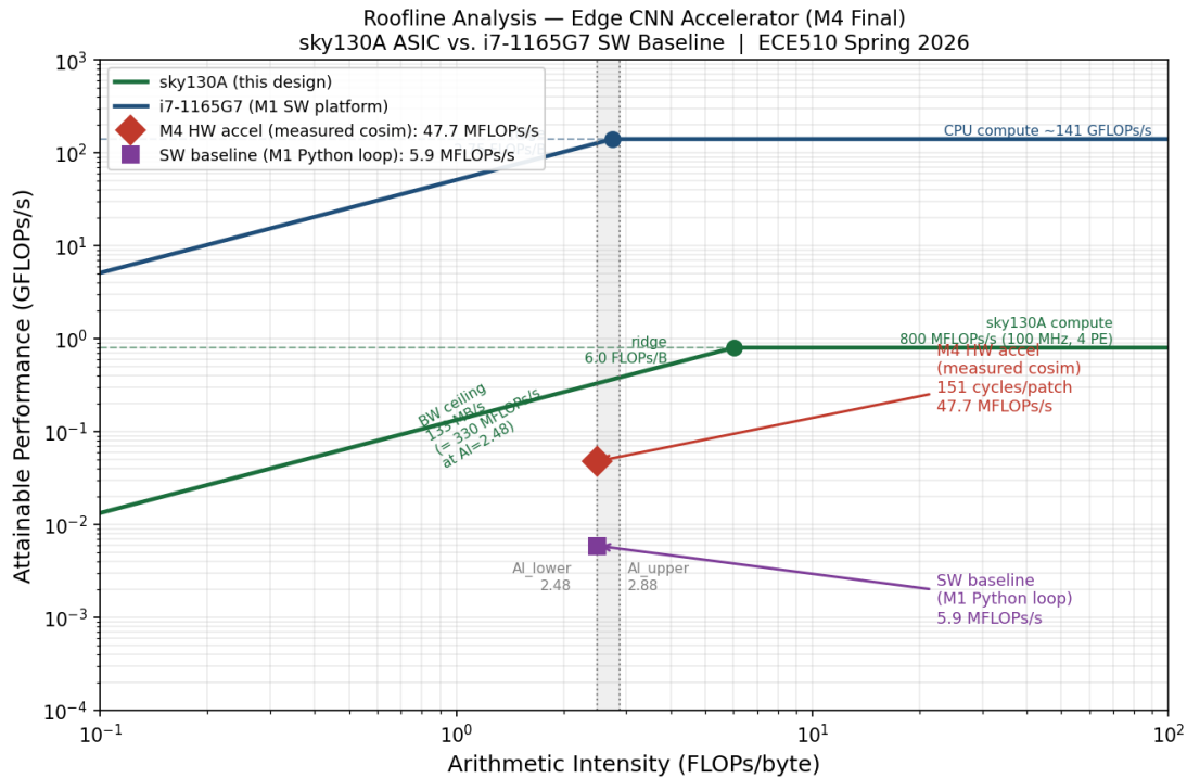
Figure 4: Roofline plot — M4 measured HW point (47.7 MFLOPs/s, 151 cycles/patch) at AI=2.48 FLOPs/byte on sky130A. SW baseline (5.91 MFLOPs/s) and sky130A roofline shown for reference.
