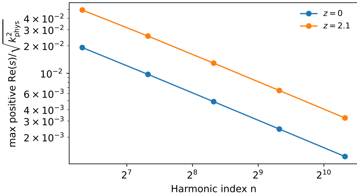
High- k positive-growth convergence
