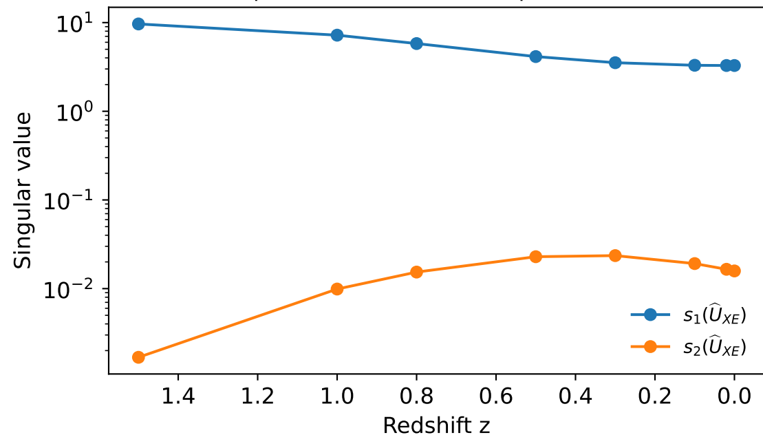
Sampled environmental temporal transfer
