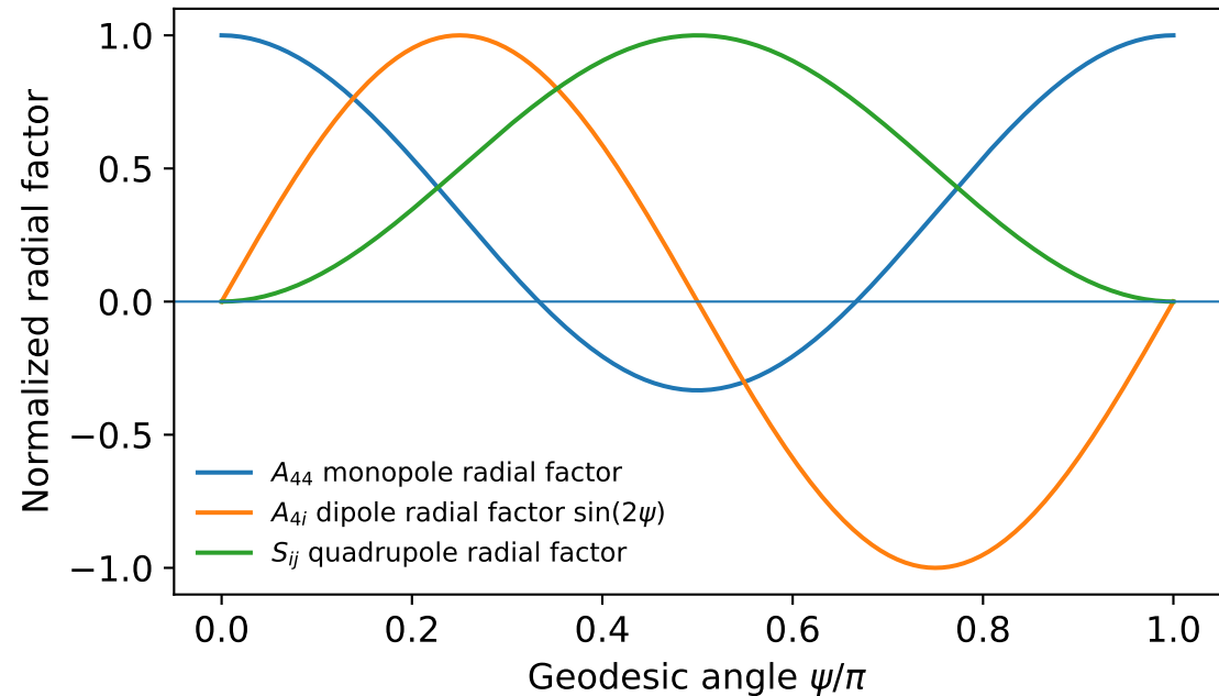
Exact n = 2 observer-shell radial factors
