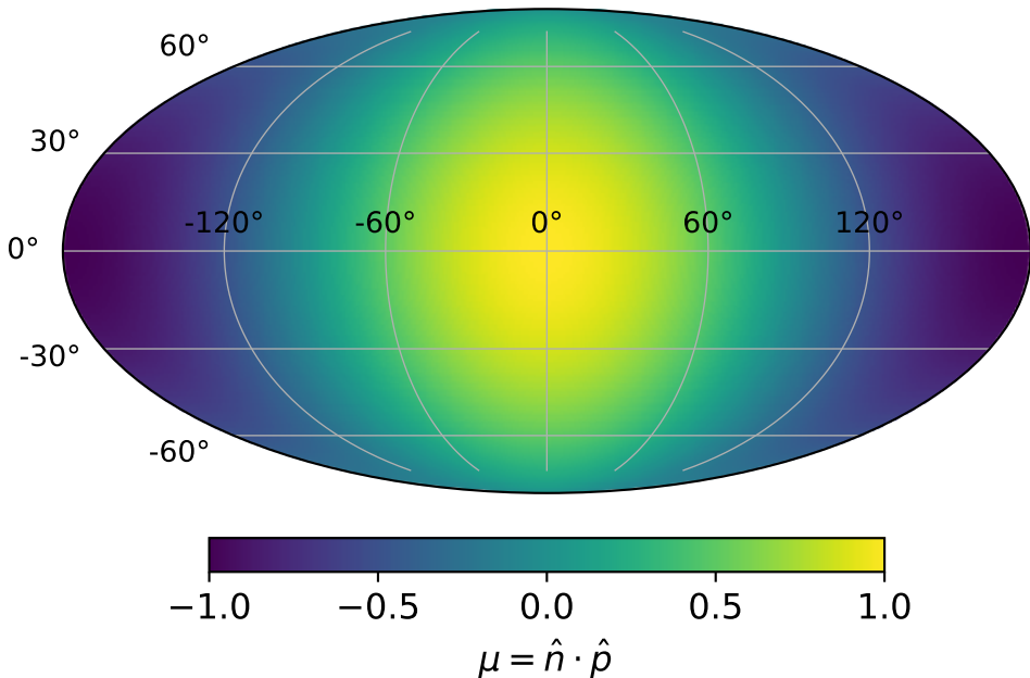
Pure A_{4i} observer-sky factor ( \hat{n} \cdot \hat{p} )
