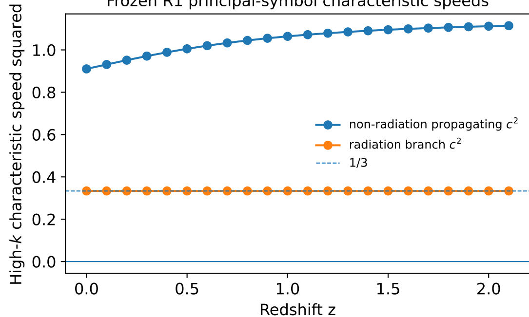
Frozen R1 principal-symbol characteristic speeds
