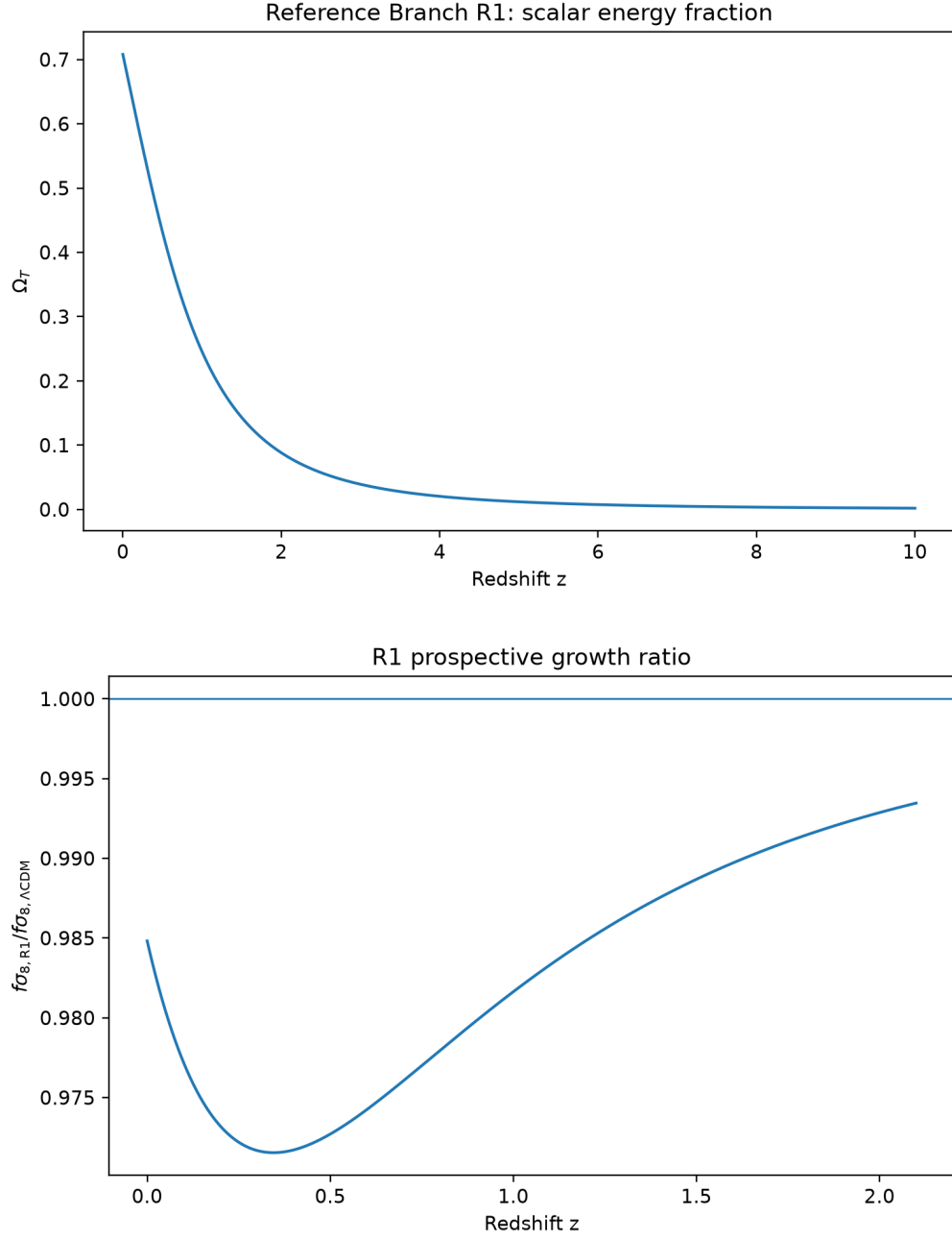
Figure 4: Conditional frozen R1 background: scalar energy fraction (top) and growth ratio (bottom), relative to matched curved \Lambda CDM with identical early normalization. These are reference calculations, not fits or survey-window RSD likelihoods. Near-standard high- n recovery is conditional on the illustrative retained filter.
