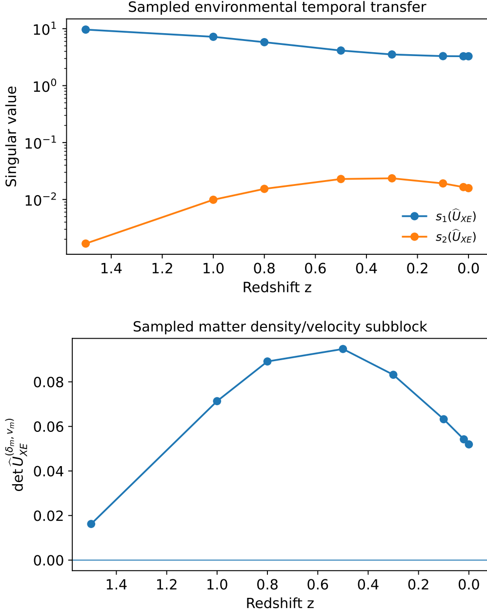
Figure 3: Environmental transfer in the (\zeta, \dot{\zeta}) output basis: singular values of \hat{U}_{XE} (top) and its matter-density/velocity subblock determinant (bottom). Points are the eight audited post-anchor epochs; lines only guide the eye. Both temporal components are accessible there. Singular-value magnitudes depend on coordinate normalization; rank is unchanged by the positive conversion to (q_2, \Pi_2) . The block vanishes at the anchor, which is not plotted. This is not spatial profile or axis selection.
