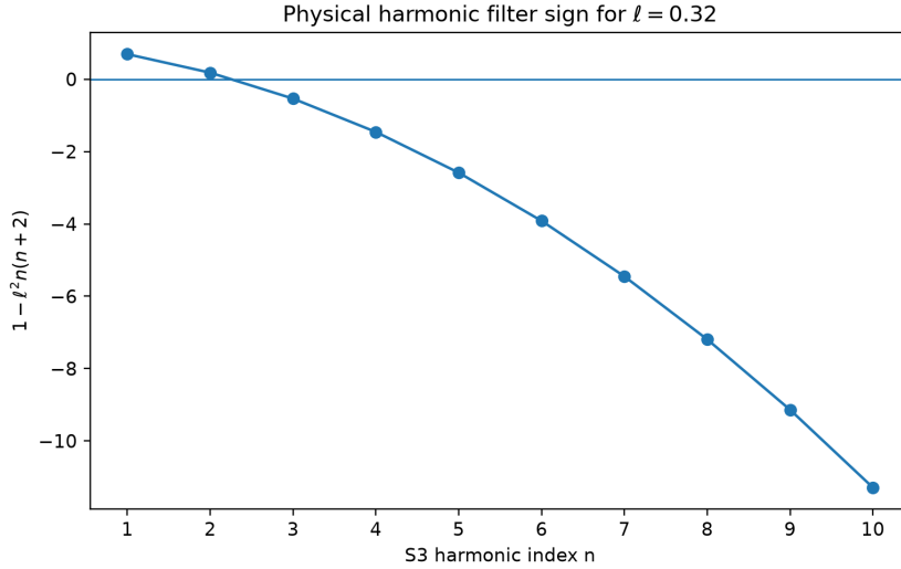
Figure 8: Sign of the Schur-response factor 1 - \ell^2 n(n+2) for the illustrative filtering value \ell = 0.32 , matching the canonical code. The physical n = 2 branch is softened and n \geq 3 stiffened; the displayed n = 1 coefficient is exceptional and excluded from propagation.
