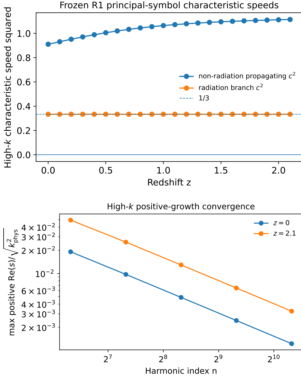
Figure 5: Frozen R1 coupled principal-symbol audit. Top: extrapolated characteristic speed squares at the audited redshifts, including the radiation 1/3 reference. Bottom: the positive normalized growth tail at the two redshift endpoints decreases across the retained high- n sequence. A positive finite- n tail is not erased; convergence is numerical evidence within the audited quadratic domain, not an all-scale stability theorem.
