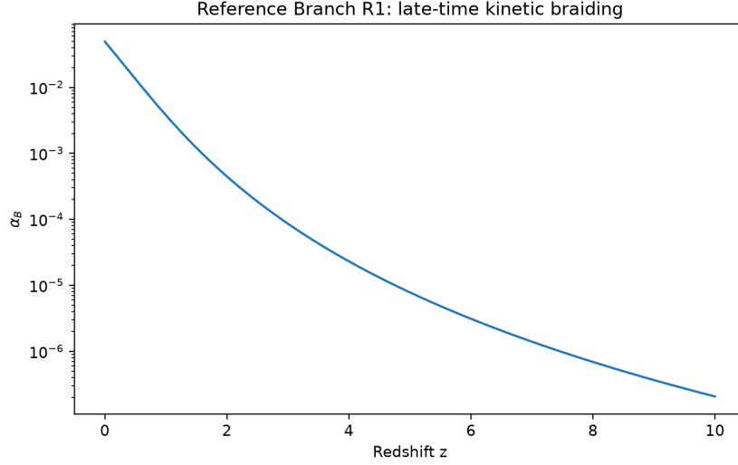
Figure 7: Conditional reference calculation, not an observational fit: kinetic-braiding function \alpha_B(z) for Reference Branch R1. The logarithmic vertical scale emphasizes the suppression of the braiding sector toward high redshift.
