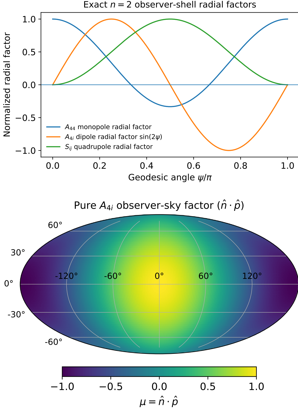
Figure 2: Exact n = 2 observer-shell radial factors (top) and the pure A_{4i} angular dipole (bottom). The plotted axis is centered solely for visualization; no empirical RA/Dec, amplitude or redshift law is used. A general trace-free 4 \times 4 tensor has nine independent components; the pure dipole is a conditional subspace.
