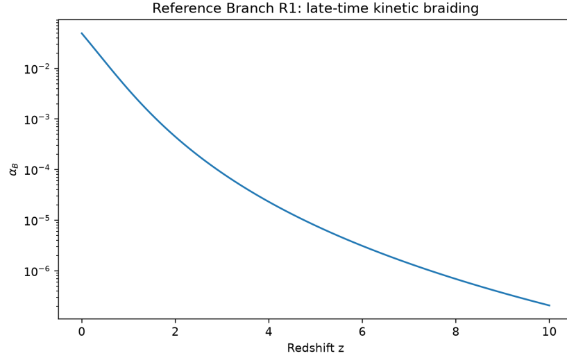
Figure 3: Conditional reference calculation, not an observational fit: kinetic-braiding function \alpha_B(z) for Reference Branch R1. The logarithmic vertical scale emphasizes the suppression of the braiding sector toward high redshift.
