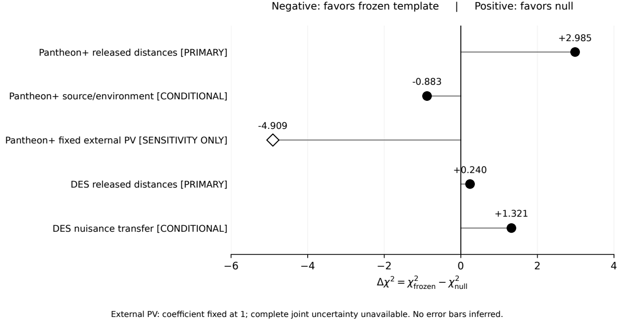
Figure 2: Five frozen comparisons on a common dimensionless scale, regenerated from the saved likelihood table. Negative model-minus-null changes favor the frozen template. The hollow diamond denotes sensitivity only: external PV mean fixed at coefficient 1; complete joint uncertainty propagation unavailable. These are likelihood changes, not significance estimates or measurements with error bars. Sample sizes and conditional mock tails are in Table 4.
