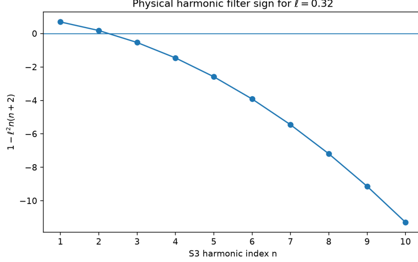
Figure 5: Sign of the Schur-response factor 1 - \ell^2 n(n+2) for the illustrative filtering value \ell = 0.32 , matching the canonical code. The physical n = 2 branch is softened and n \geq 3 stiffened; the displayed n = 1 coefficient is exceptional and excluded from propagation.
