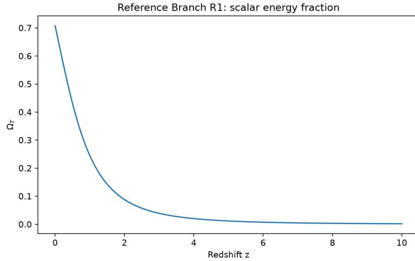
Figure 4: Conditional reference calculation, not an observational fit: scalar energy fraction \Omega_T(z) for R1. The scalar component is subdominant at high redshift and becomes dynamically important only at late times.
