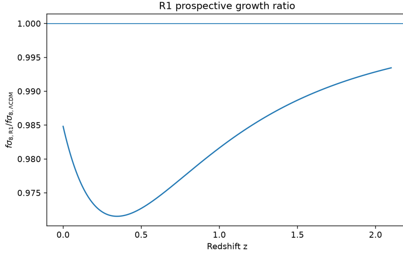
Figure 6: Prospective R1 growth ratio relative to a matched curved- \Lambda CDM background with the same early normalization.
