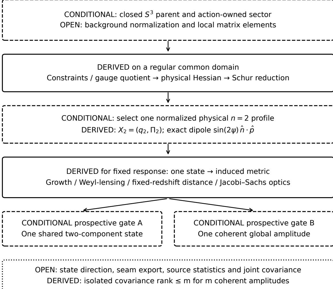
Figure 1: Constraint-to-prediction chain. Solid, dashed and dotted boxes identify DERIVED identities, CONDITIONAL physical choices, and OPEN inputs; status is also written in every box. A single selected state feeds all observable rows. No independent observable amplitude is introduced.
