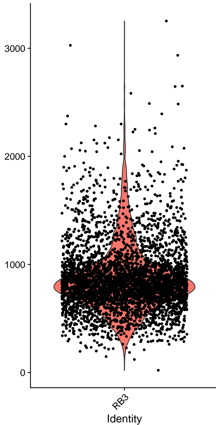
nFeature_RNA
