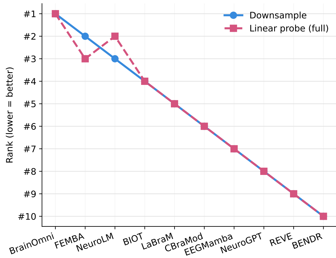
Rank consistency across evaluation settings (Spearman \rho = 0.988 )
