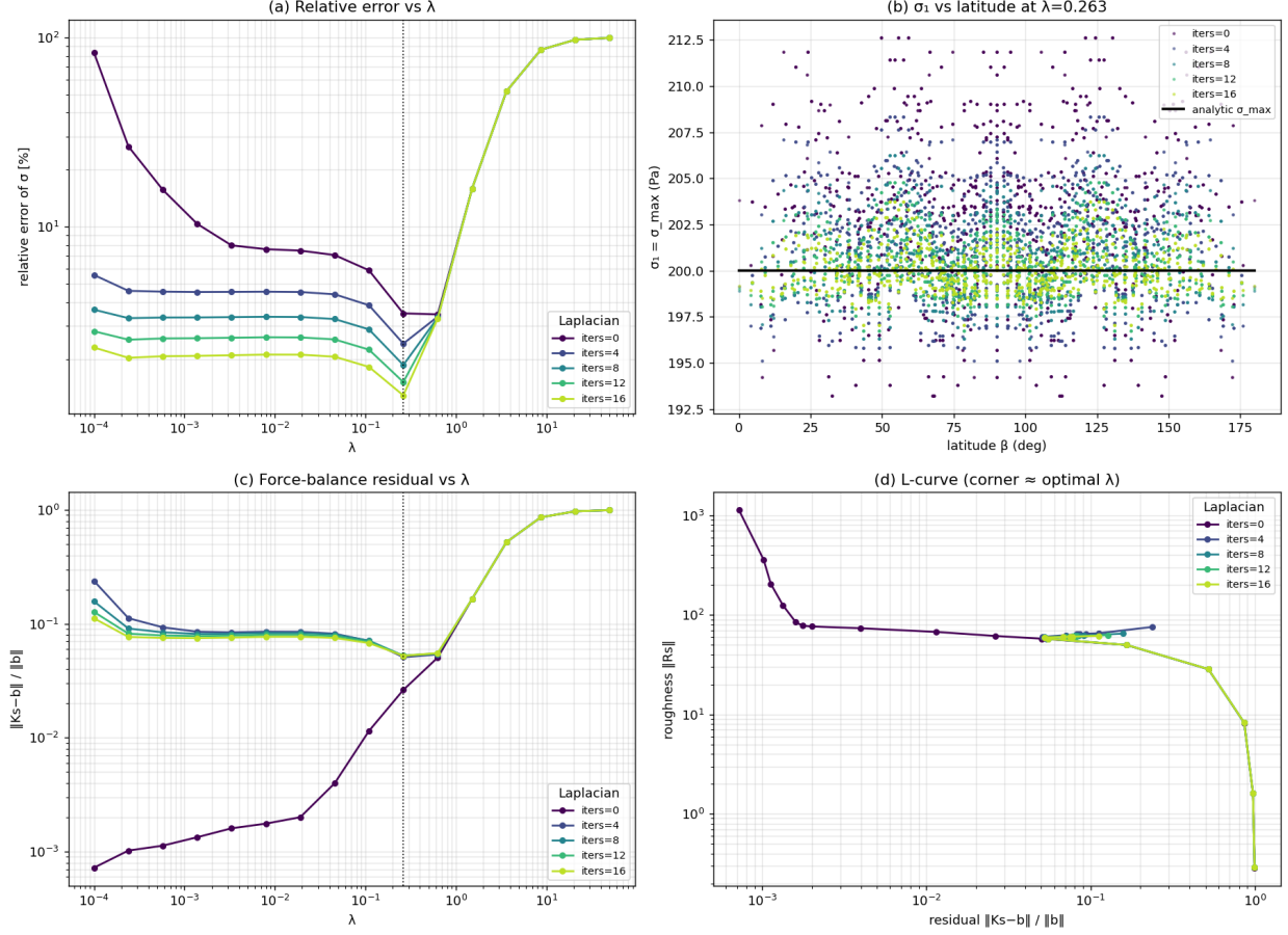
Figure 7: Sphere. Joint \lambda \times Laplacian-iters sweep of the stress FEM (subdiv-4, \Delta p = 20 Pa, t = 0.05 , \alpha = 0.5 ). The sphere is the lone shape on which smoothing helps (3.45% \rightarrow 1.29%): its exact field is constant isotropic, so there is no genuine signal for the Laplacian to flatten and more iterations monotonically reduce the spurious anisotropy in panel (b).
