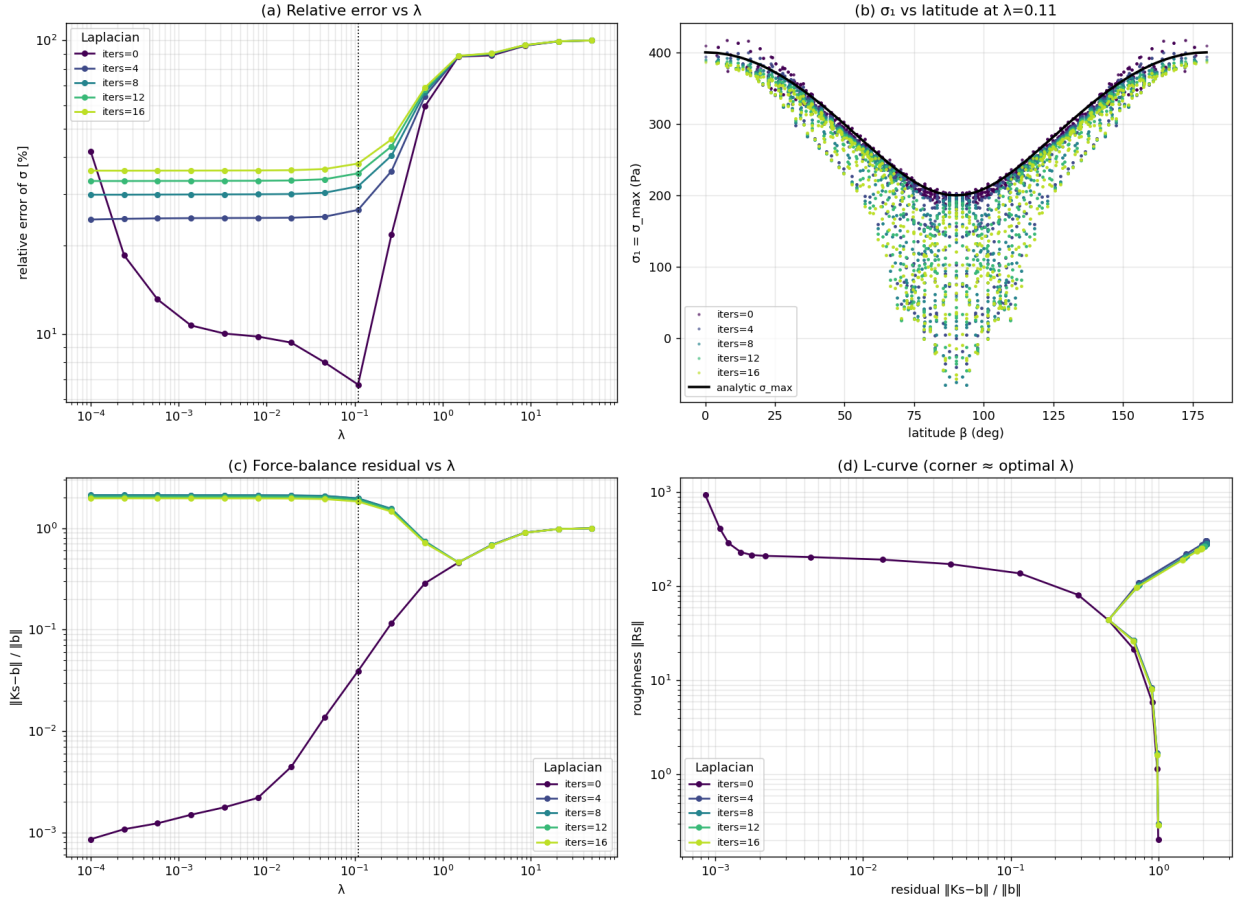
Figure 9: Oblate spheroid 1:2. As for the prolate case the optimum is at m=0 (6.72%); the larger floor reflects the stronger curvature gradients of the oblate shape, not the regularizer.
