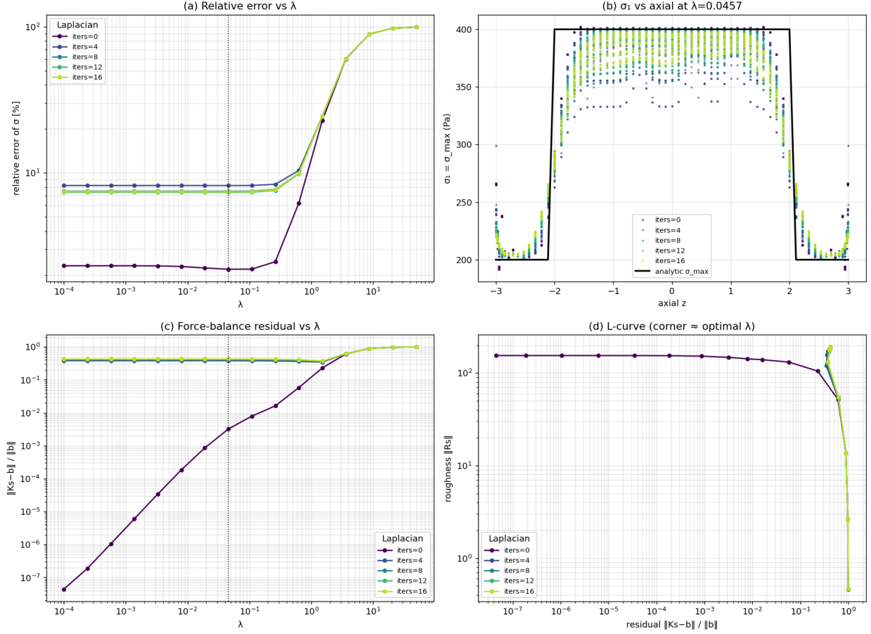
Figure 10: Capsule (cylinder R=1 , half-height H=2 , hemispherical caps). Panel (b) shows the hoop/axial step — \sigma_{\max} \approx \Delta p R/t on the cylinder body, \Delta p R/2t on the caps — which the m=0 solution (2.19%) tracks most faithfully; smoothing rounds off the step.
