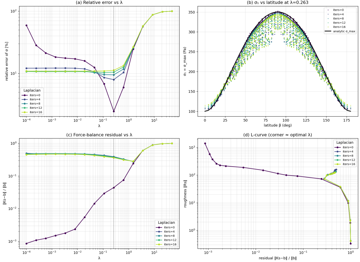
Figure 8: Prolate spheroid 2:1. The Tikhonov-only curve ( m=0 , dark) attains both the lowest error (2.47%) and the lowest residual; every smoothing pass flattens the genuine meridional/hoop variation visible in panel (b) and raises the residual in panel (c).
