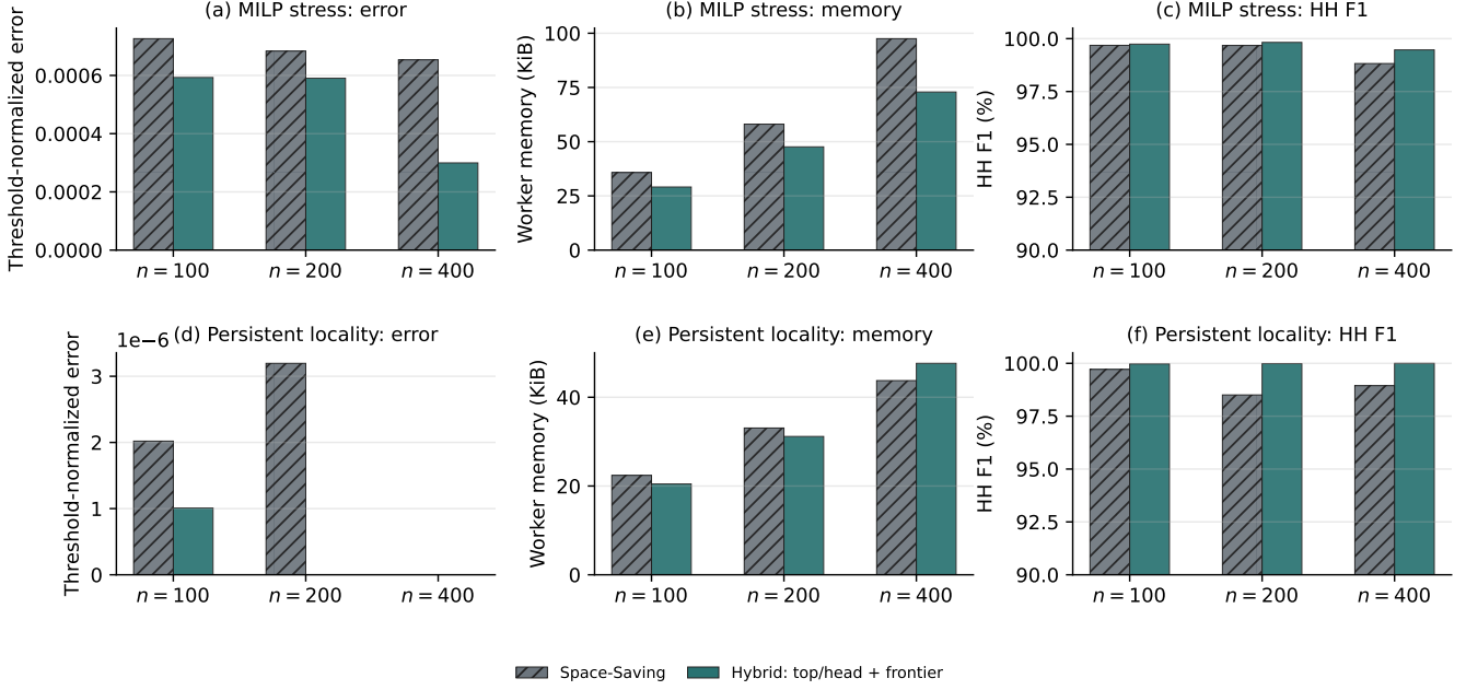
Figure 8: Hybrid exact-approximate tracking compared with the complete approximate controller. The hybrid variant promotes \text{Top}_n^t \cup K_\dagger^t \cup K_\dagger^t into exact counters for the next window and sketches only the residual tail. Error is n \cdot \text{AAE}/N , memory is mean worker memory, and HH F1 is reported in percent.
