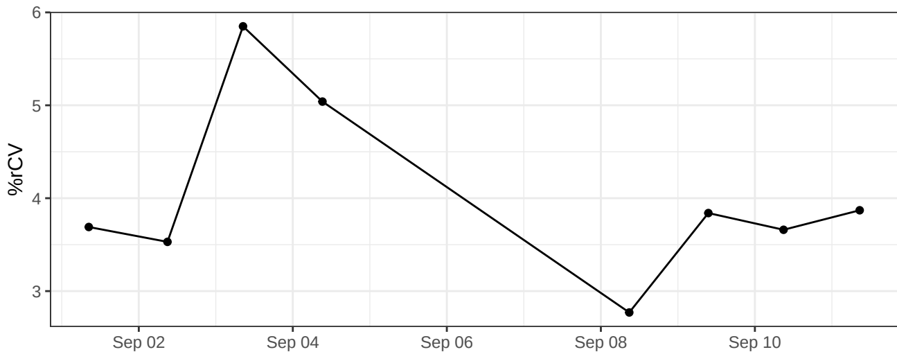
APC-A-% rCV
