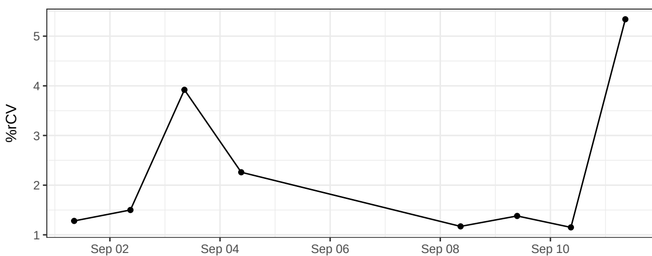
BB515-A-% rCV
