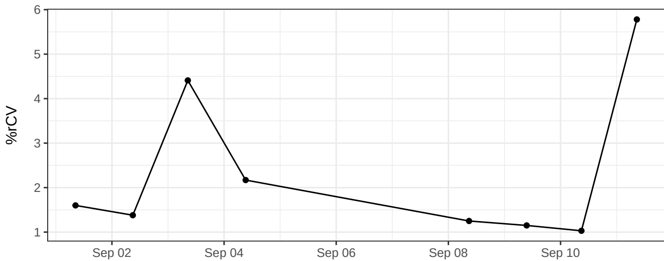
BV786-A-% rCV
