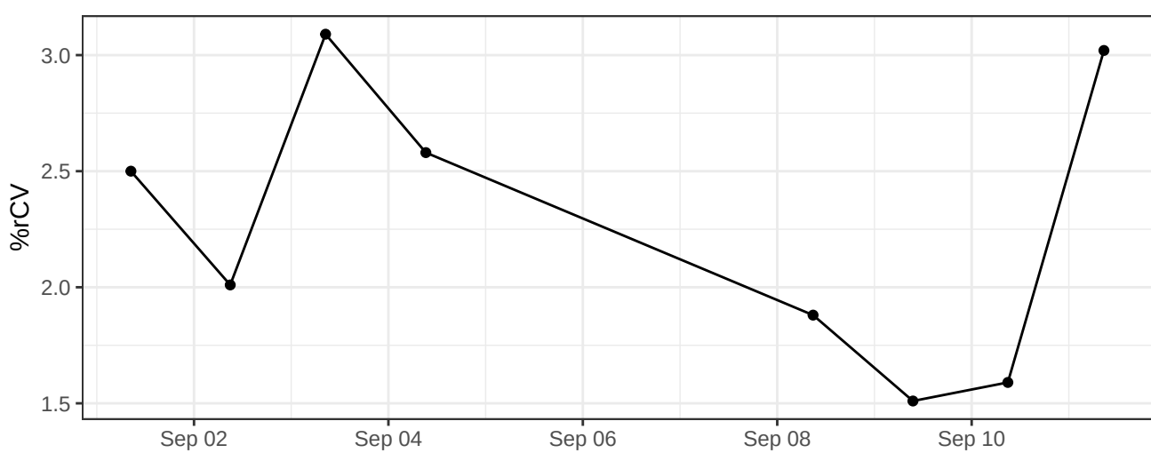
BB515-A-% rCV
