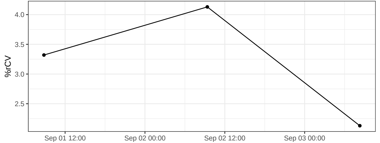
PE-A-% rCV
