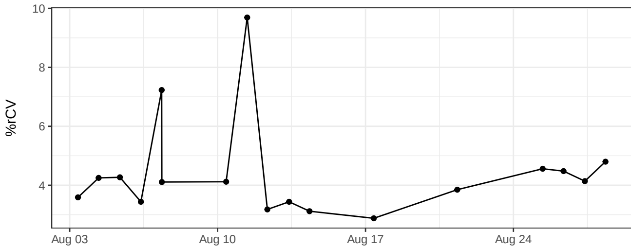
PE-Cy7-A-% rCV
