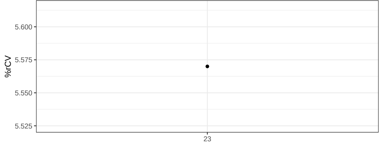
BV421-A-% rCV
