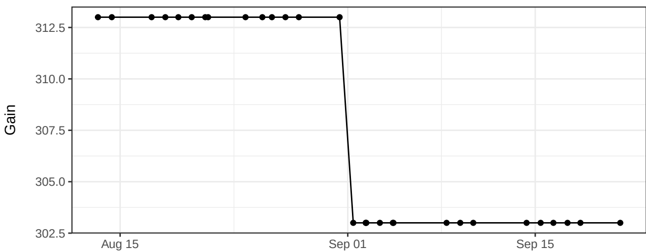
PerCP-Cy5 5 Blue-A_Gain
