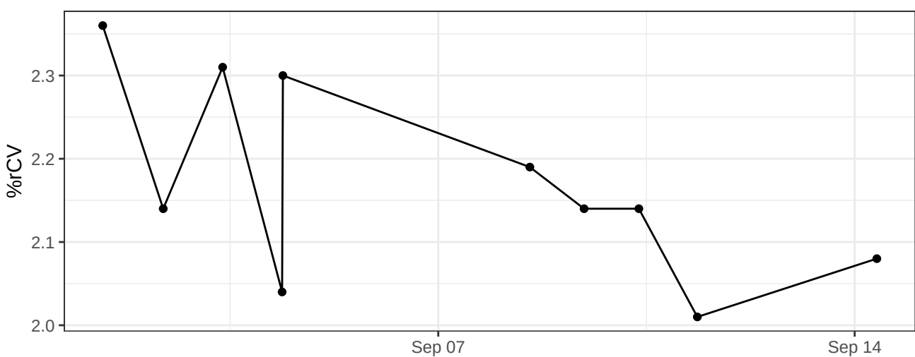
PE-CF594-A-% rCV
