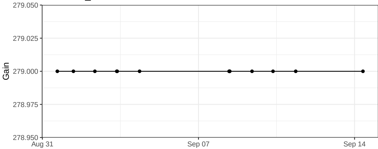
BV750-A_Gain
