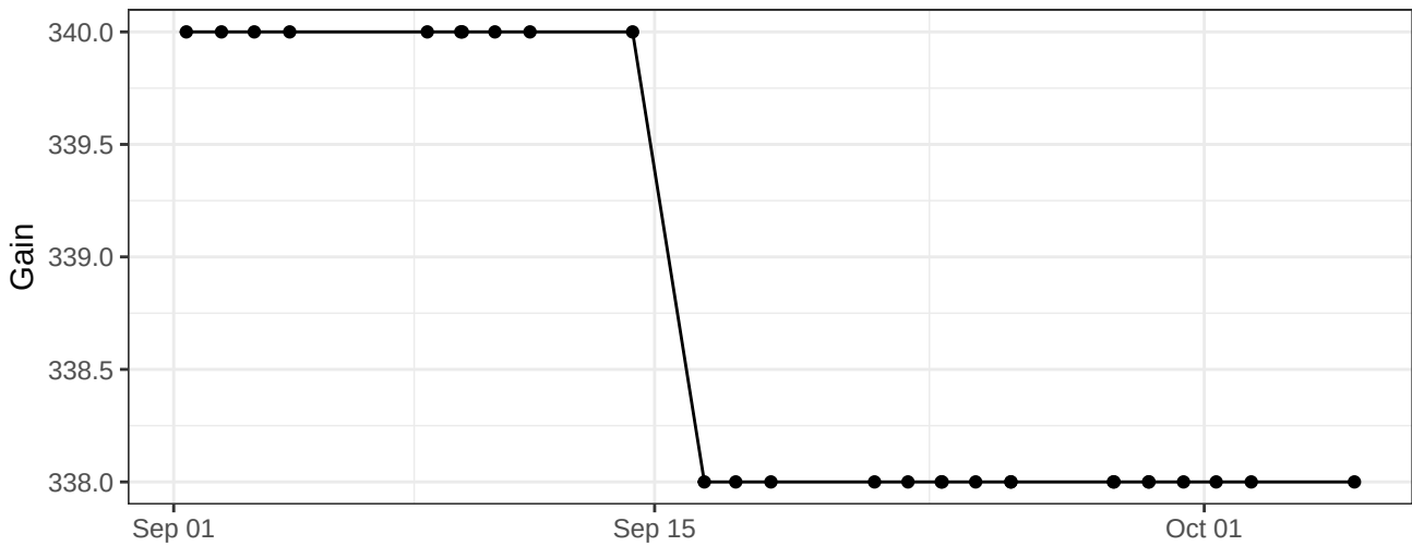
BV510-A_Gain
