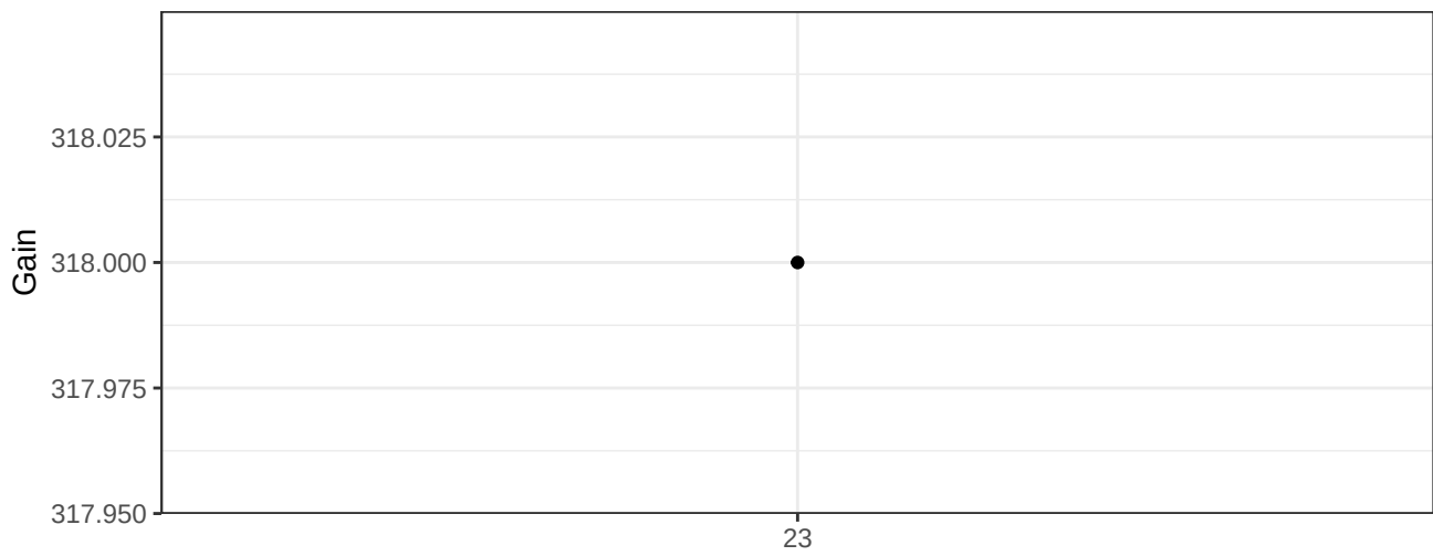
APC-A_Gain
