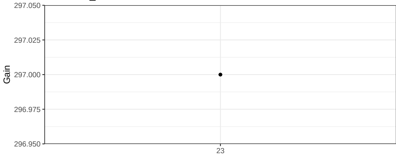
BV605-A_Gain
