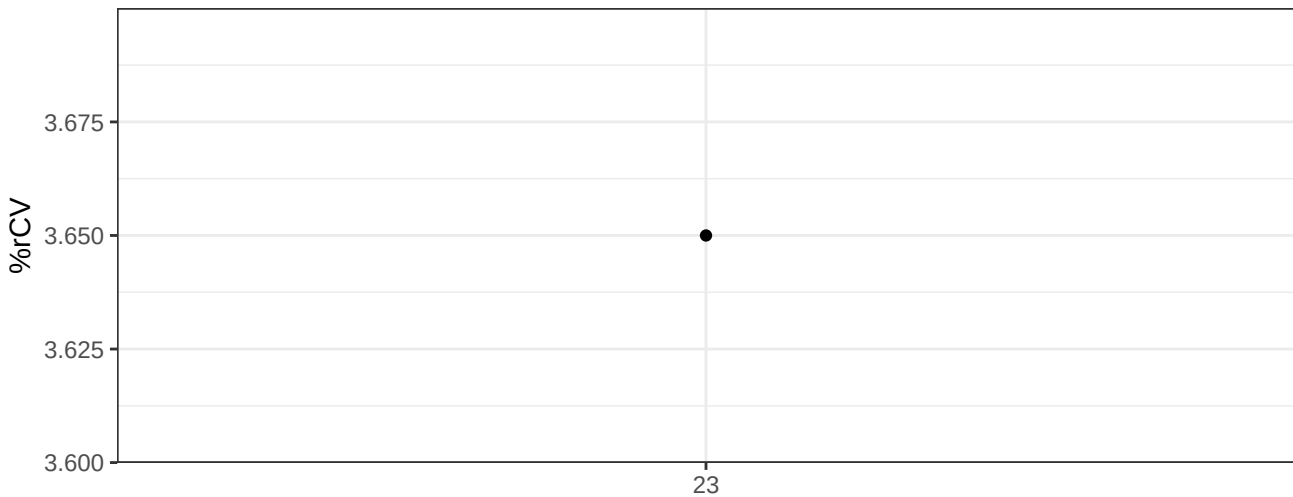
FSC-A-% rCV
