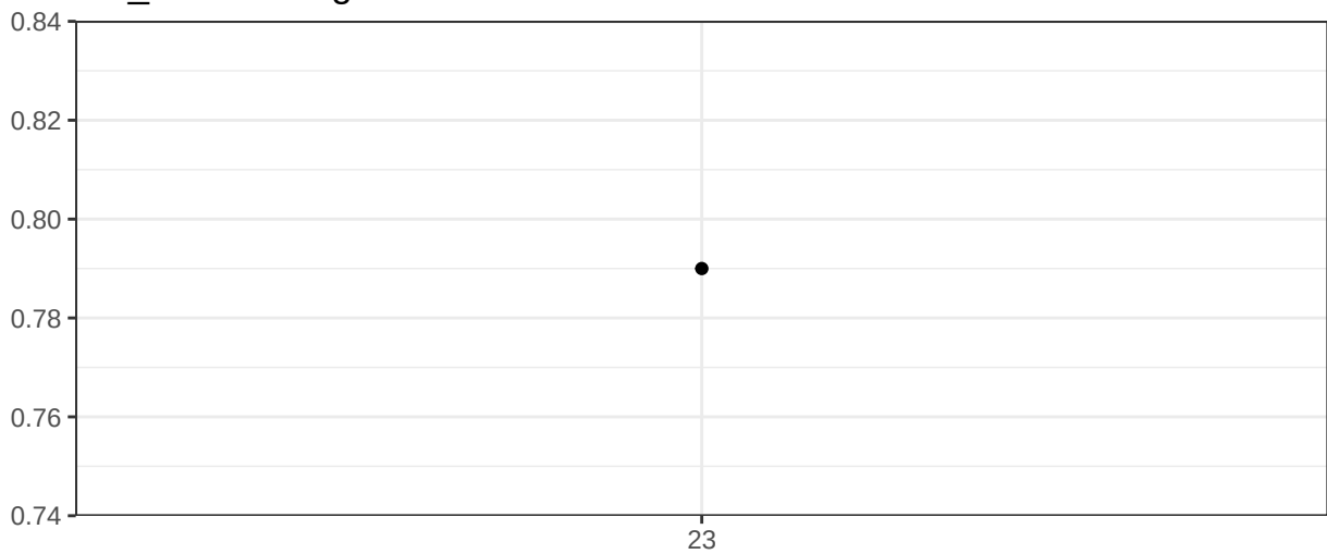
Violet_AreaScalingFactor
