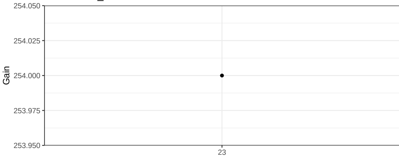
DAPI-A_Gain
