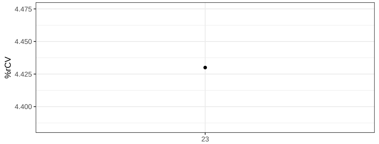
BV605-A-% rCV
