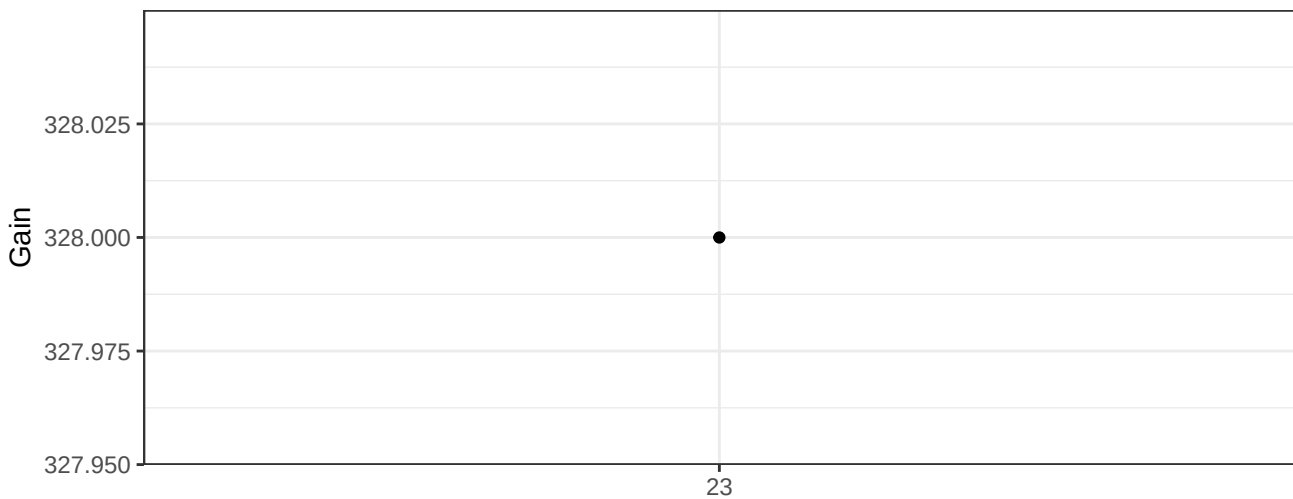
BV421-A_Gain
