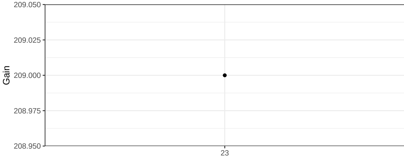
BV510-A_Gain
