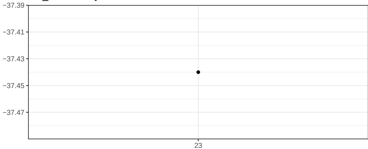
UV_LaserDelay
