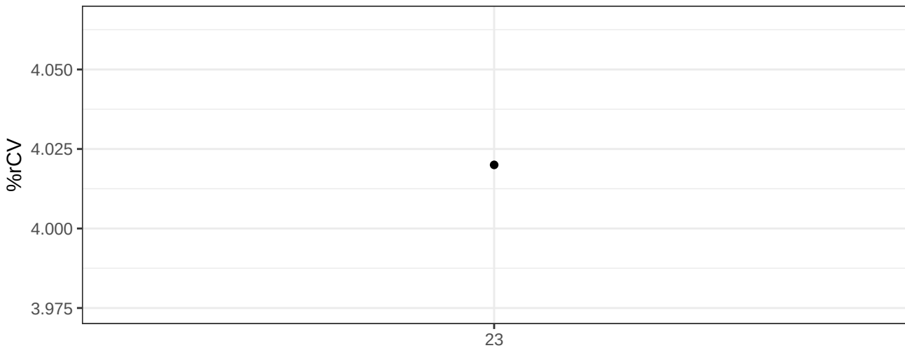
APC-A-% rCV
