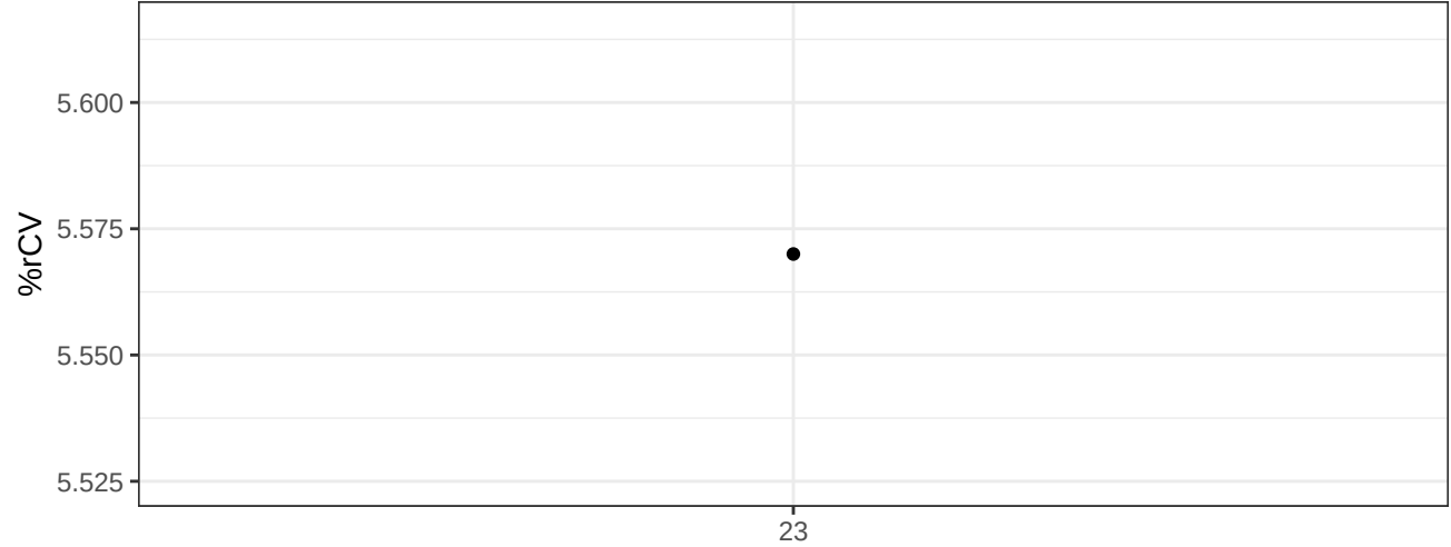
BV421-A-% rCV
