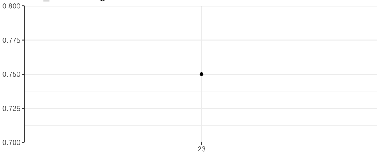
YG_AreaScalingFactor
