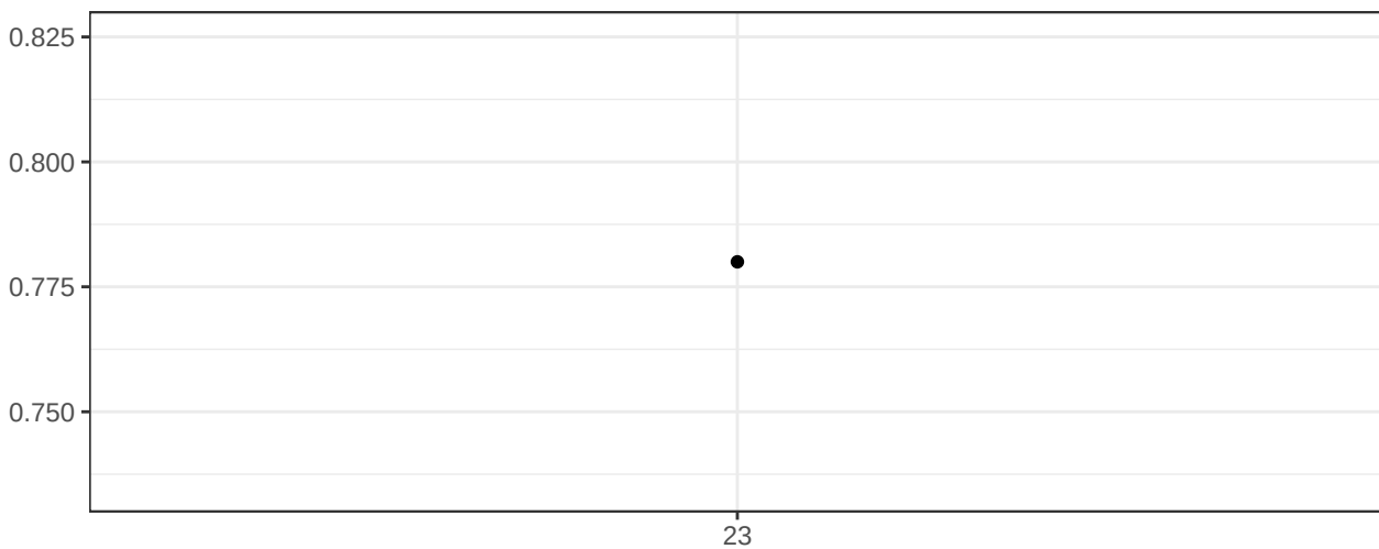
YG_AreaScalingFactor
