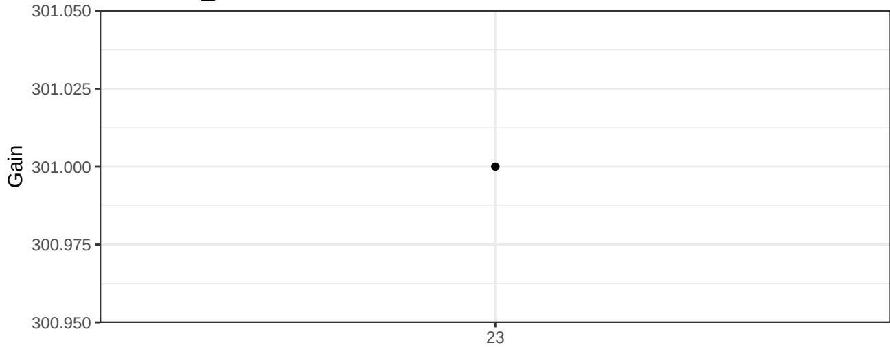
BV650-A_Gain
