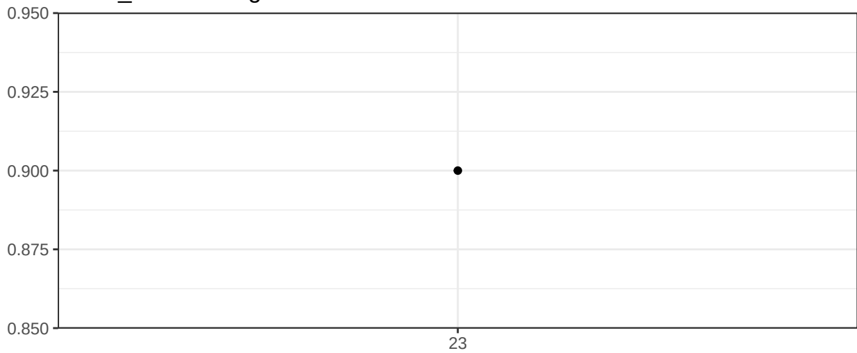
Violet_AreaScalingFactor
