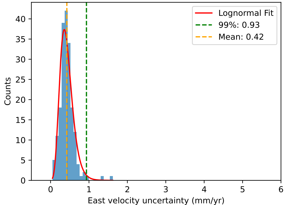
viltres_2022: East Velocity Uncertainty
