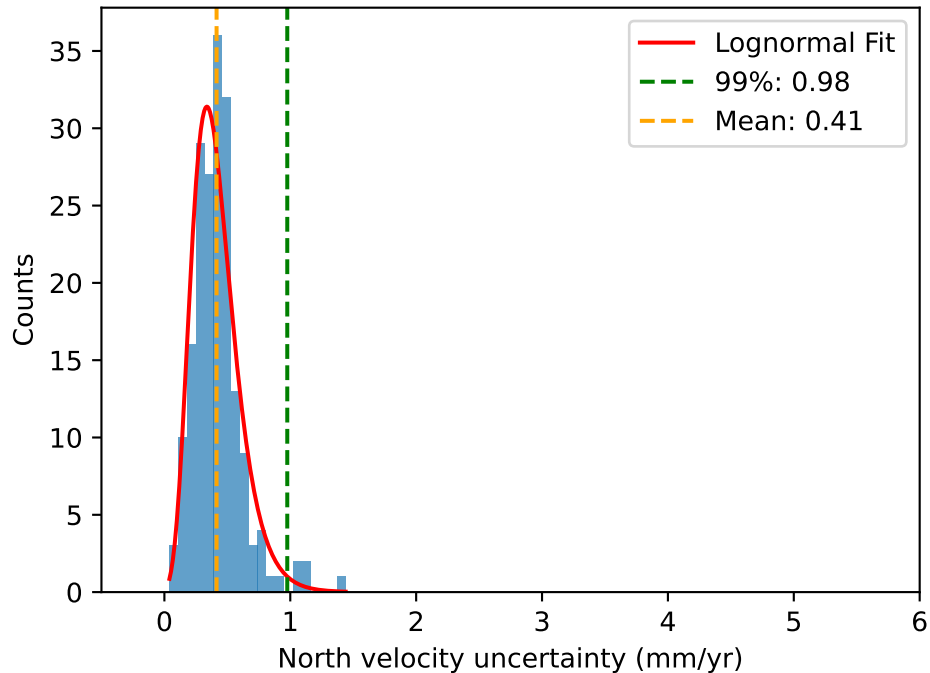
viltres_2022: North Velocity Uncertainty
