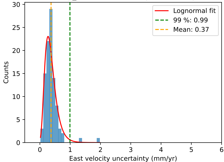
ozbey_2024: East velocity uncertainty
