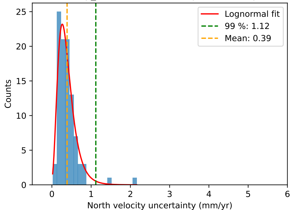
ozbey_2024: North velocity uncertainty
