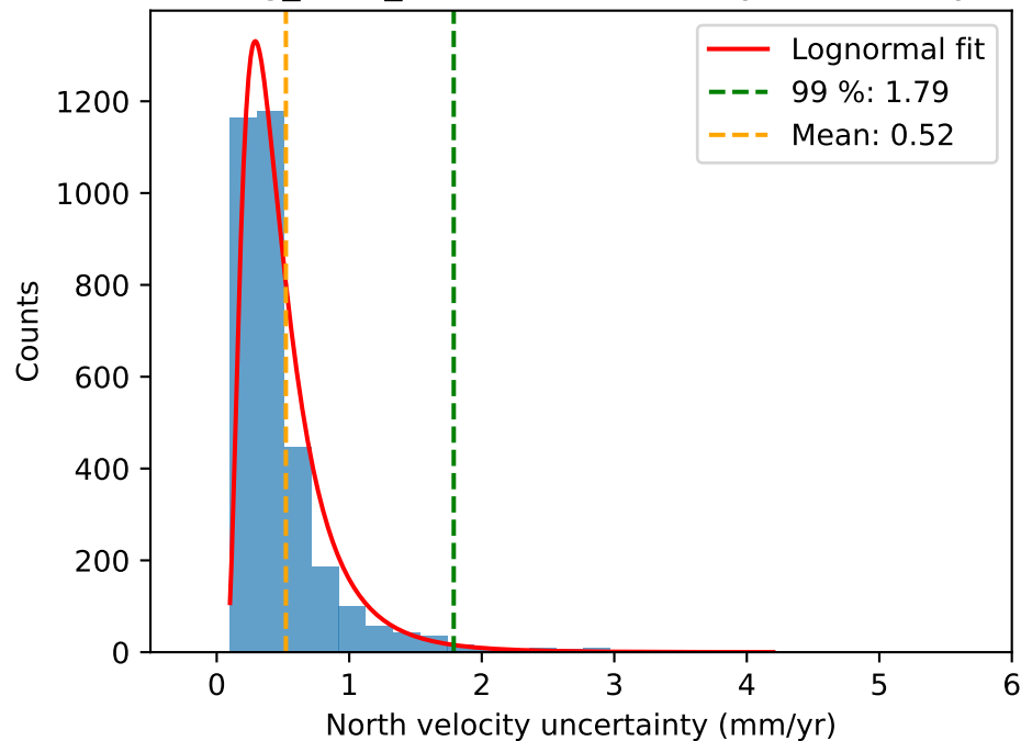
wang_shen_2020: North velocity uncertainty
