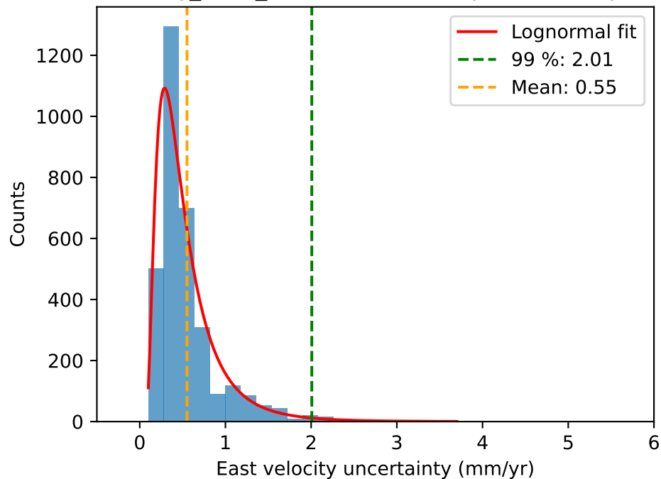
wang_shen_2020: East velocity uncertainty
