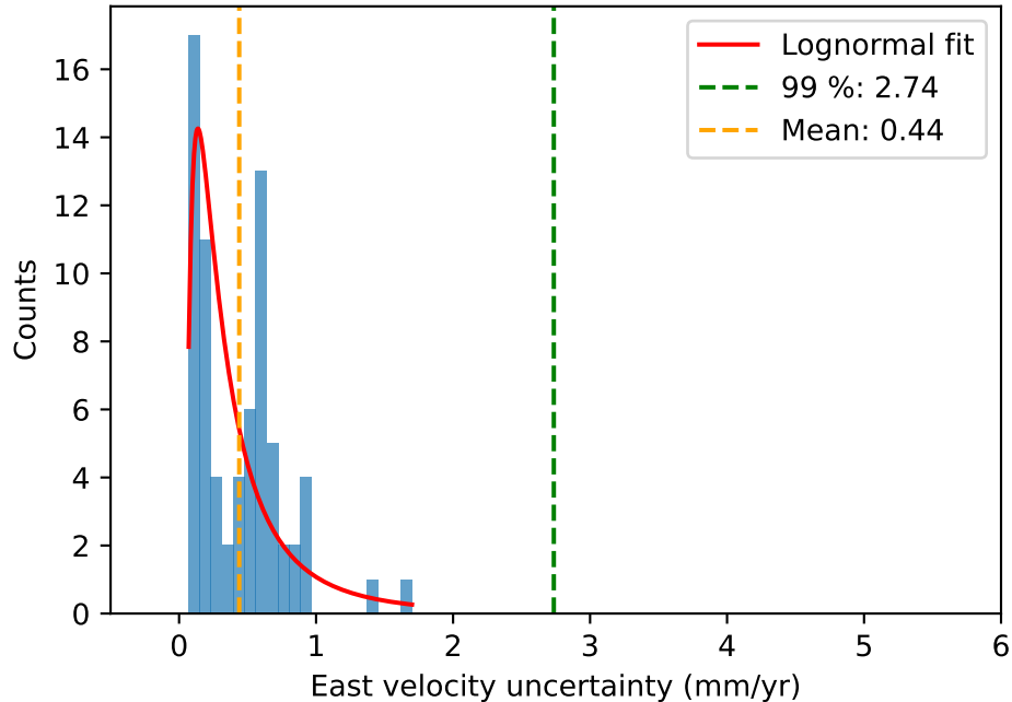
sokhadze_2018: East velocity uncertainty
