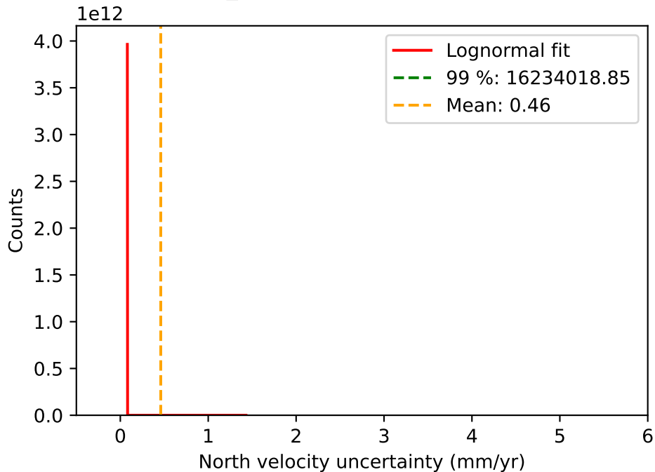
sokhadze_2018: North velocity uncertainty
