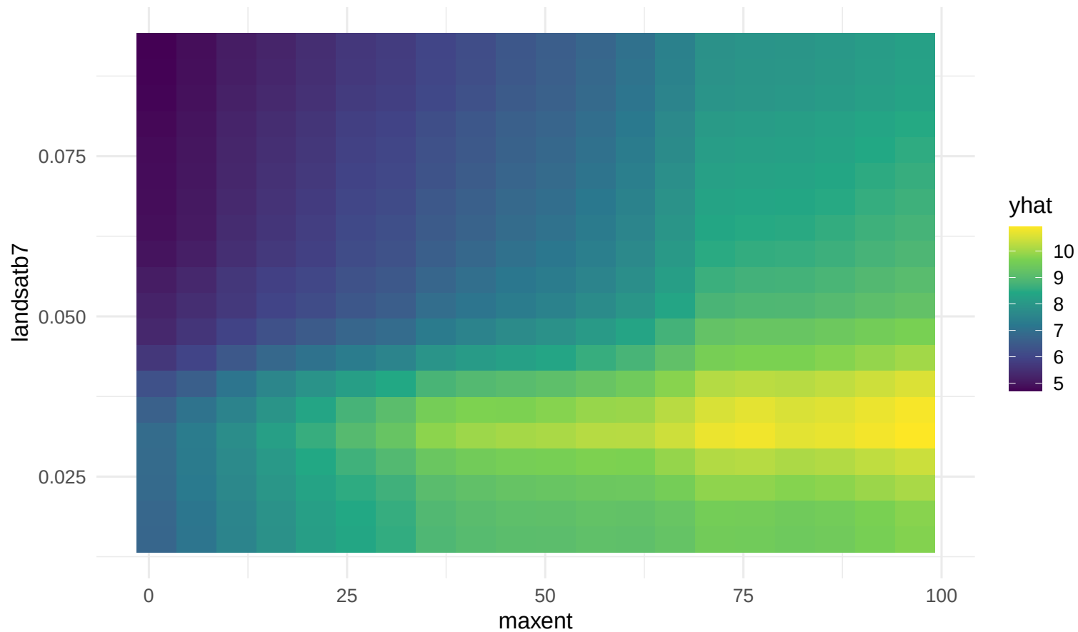
2-Way Partial Dependence: maxent \times landsatb7
