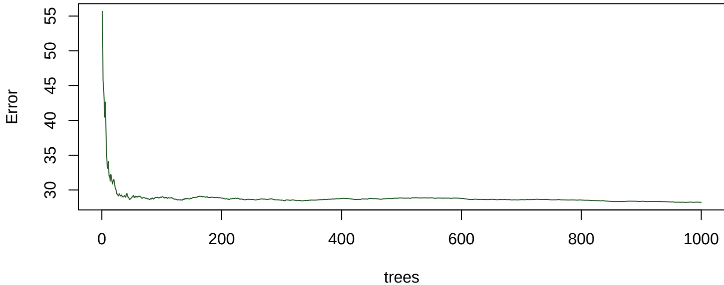
OOB Error vs Number of Trees (Otot)
