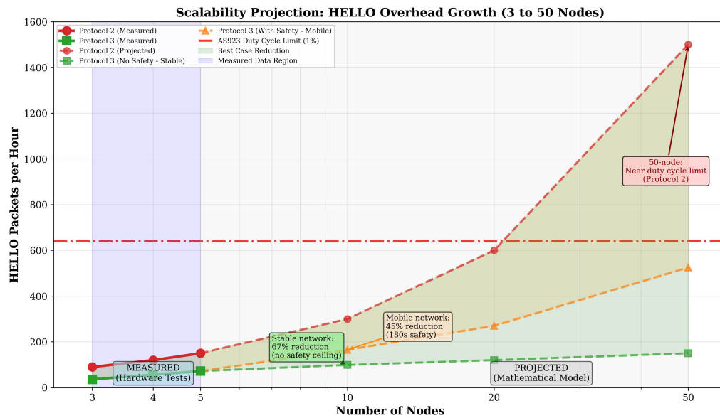
Figure 5.1: Scalability Projection – HELLO Overhead Growth
